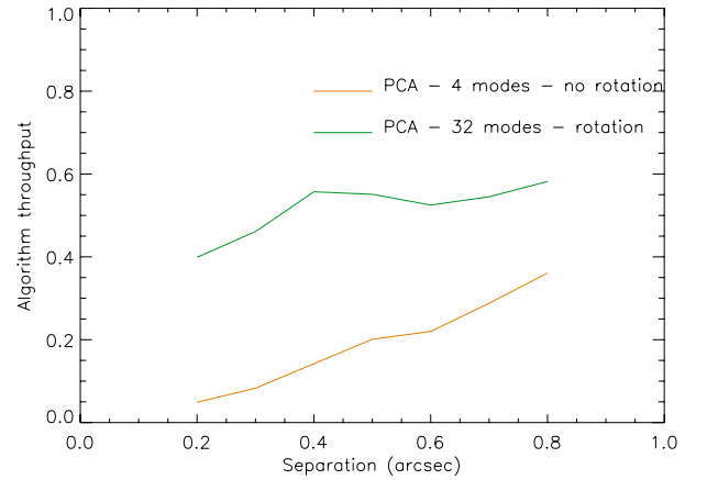
Fig. 13. Algorithm throughput versus separation for two sets of the PCA method parameters. The algorithm throughput is represented by the orange curve and corresponds to no rotation of the FOV and 4 principal components, as shown in Fig. 11 while the green line represents the FOV rotation case and 32 principal components as shown in Fig. 12.
