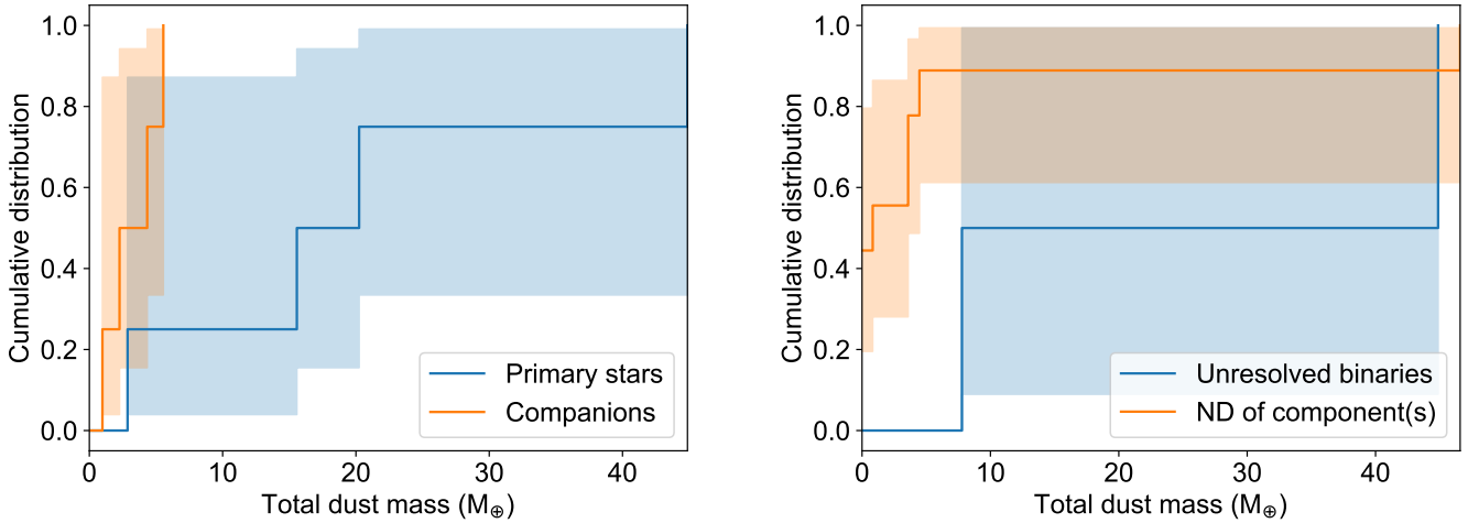
Figure 6. Cumulative distribution of the total mass of the dust in the primaries vs the companions as measured in the ALMA data.
