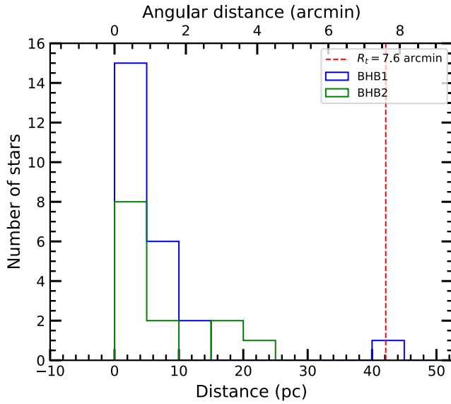
Figure 4. The radial distribution of UVIT detected BHBs. The histogram of BHB1 stars is shown in blue line and histogram of BHB2 stars is shown in green line. The lower and upper x-axes is the distance from the cluster center in parsec and arcminutes, respectively. The y-axis represents the number of stars present in each distance bin of 5 parsec from the cluster center. The vertical dashed line is the tidal radius of the cluster.
