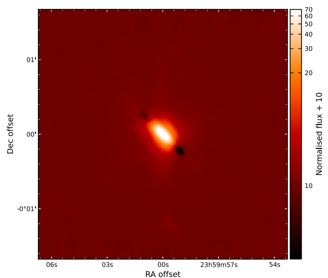
Figure 1. Image of Vesta taken in parallel mode with a scan speed of 60 arcsec s -1 and array-to-map inclination angle of \alpha = 42.5 showing the details of the PSF. In order to use a logarithmic stretch, a constant value of 10 was added to the normalized fluxes.
