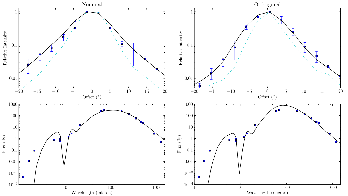
Figure 8. The combined best-fitting model (solid black) in terms of the 70 \mu\text{m} scan profile (top) and SED (bottom) compared to the data (blue squares) for G030.8185+00.2729. The left-hand panels are for the scan in the nominal direction whilst the right-hand panel is for the scan in the orthogonal direction. The Vesta PSF scan is shown in the top panel (dashed cyan) to illustrate the extended nature of the MYSO emission. An error of 10 per cent of the total observed fluxes was considered in the observed SED.
