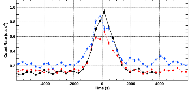
Figure 10. Light curves, in the 2-10 keV band, of the three brightest XMM-Newton flares, VB1, VB2 and VB3 are shown with back squares, red circles and blue stars, respectively. The light curves of the three very bright flares observed by XMM-Newton show very similar time evolution and comparable duration. These light curves are the result of the sum of the data from EPIC-pn and MOS. For display purposes, we shifted the time axis aligning the peak of the Gaussian best fitting the flare profile (see Tab. 7).
