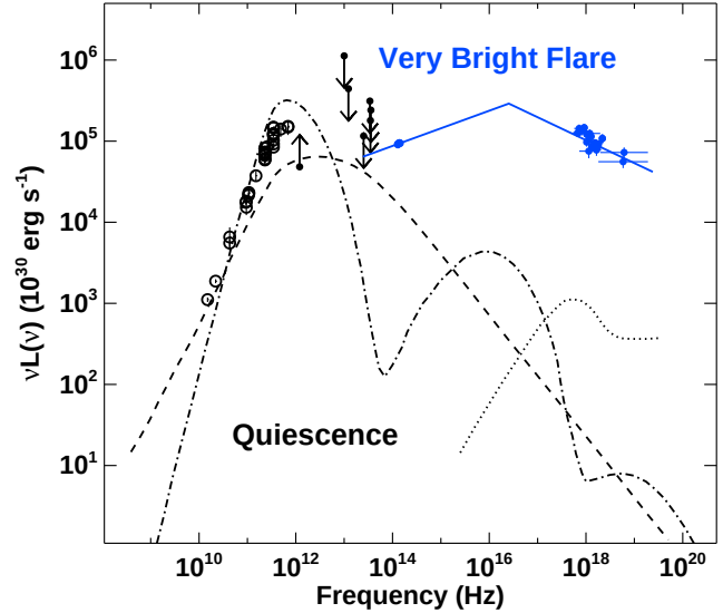
Figure 1. Multi-wavelength emission from Sgr A*. The radio to mid-IR data points (open circles as well as upper-lower limits) constrain Sgr A*'s quiescent emission (these constraints are taken from the literature, see text). The black lines show the radiatively inefficient accretion disc model proposed by Yuan et al. (2003). The dash-dotted black line shows the contribution from the thermal electrons with T_e \sim \text{few } 10^{10} \text{ K} and n_e \sim 10^6 \text{ cm}^{-3} , embedded in a magnetic field with strength of \sim 10 - 50 \text{ G} producing the sub-mm peak and (possibly) inverse Compton emission at higher energies. The dashed line shows the contribution from a non-thermal tail in the electron population, while the dotted line shows the bremsstrahlung emission from hot plasma at the Bondi radius (Quataert 2002). The blue filled data points shows the mean NIR and X-ray spectra of the very bright flare VB3 and the blue solid line shows the best fit power-law with cooling break (see also Fig. 6).
