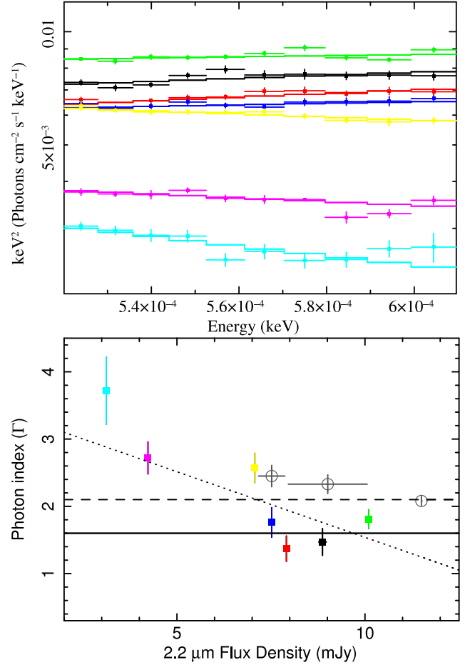
Figure 6. (Top panel) SINFONI spectra fitted with a power-law model in the energy band E \sim 0.525 - 0.608 eV. The color (black, red, green, blue, cyan, magenta and yellow) indicates the chronological sequence of the spectra. (Bottom panel) Best fit photon index ( \Gamma_{\text{NIR}} ) as a function of the 2.2\ \mu\text{m} flux density (in mJy units). The NIR photon indexes are shown with filled squares, with the same color code as before. The empty dark grey circles show the spectral indexes in the 2-10 keV band, during the rise, decay and peak of very bright flares. For these points, we associate to the flare rise and decay X-ray photon indexes the simultaneous NIR fluxes. For the flare peak, we assume a value of 11.5 mJy. The dotted lines show the best fit of the NIR photon indexes with a linear relation. The solid line shows the constant photon index typically observed at medium-high fluxes (flux density > 7 mJy; \Gamma_{\text{NIR}} = 1.6 ; Hornstein et al. 2007). The dashed line shows the associated X-ray slope, if the spectrum is dominated by synchrotron emission with a cooling break \Gamma_X = \Gamma_{\text{NIR}} + 0.5 .
