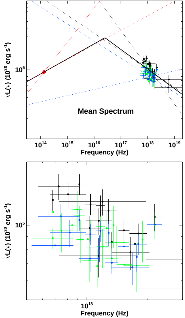
Figure B1. (Top panel) The red points show the mean NIR ( SINFONI ) during the VB3 flare, such as in Fig. 4. The blue points show the corresponding X-ray ( XMM-Newton and NuSTAR ) spectra, when no dust correction is applied. The green and black points show the X-ray spectra corrected for the effects of dust scattering according to the DUST and FGCDUST models, respectively. The stronger the correction, the brighter and steeper becomes the X-ray spectrum (see text for details). The red, blue and black dotted lines show the uncertainty on the NIR slope, on the X-ray slope when no correction for dust is applied and once the data are corrected using the FGCDUST model, respectively. The black line shows the best fit PLCool model (where the X-ray and NIR slopes are tied). All data and models and data are de-absorbed. (Bottom panel) Enlargement of the top panel into the X-ray band, to allow a better elucidation of the extent of the effect.
