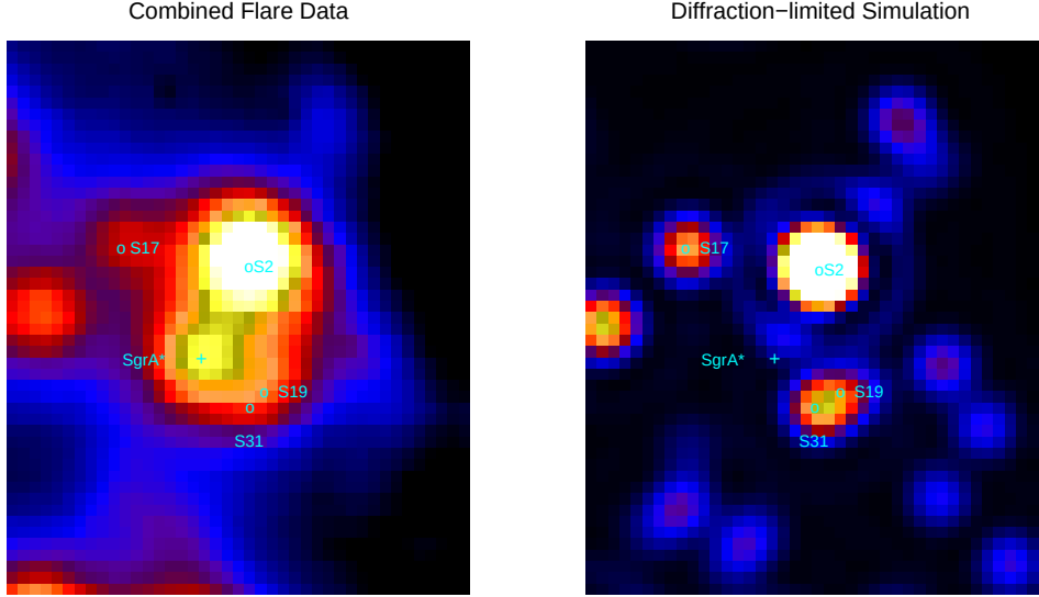
Figure 2. The GC as seen with SINFONI (each image is 0.51'' \times 0.61'' ). The image on the left is the collapsed image from the spectral range 2.25\text{--}2.35\ \mu\text{m} for the seven data cubes combined. The image on the right is a diffraction-limited simulated image of the locations of the S-stars in the GC. In both images the location of Sgr A* is indicated with a cross, and the four stars included in our Gaussian fits for spectrum extraction are labeled with circles. The flare is clearly visible above the background in the left image.
