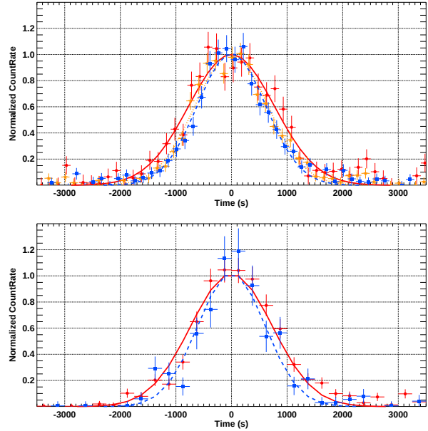
Figure 12. ( Upper panel ) The combination of the light curves of VB1, VB2 and VB3 in the 2-4 keV (red squares), 4-6 keV (orange stars), 6-10 keV (blue squares), light curves are shifted by the center of their best-fit Gaussian profile, subtracted by the best-fit local underlying continuum, and normalised by the peak of their best-fit Gaussian. Time bins of 150 s are used. Flares are shorter in the hard band. ( Bottom panel ) Chandra composite light curve for 2-4.5 keV (red circles) and 6-9 keV (blue squares). All bright flares not significantly affected by pile-up (peak count rate < 0.1 ph s ^{-1} ) are considered here. The light curves are shifted with the same method described above. Time bins of 250 s are used. Flares last longer in the soft band.
