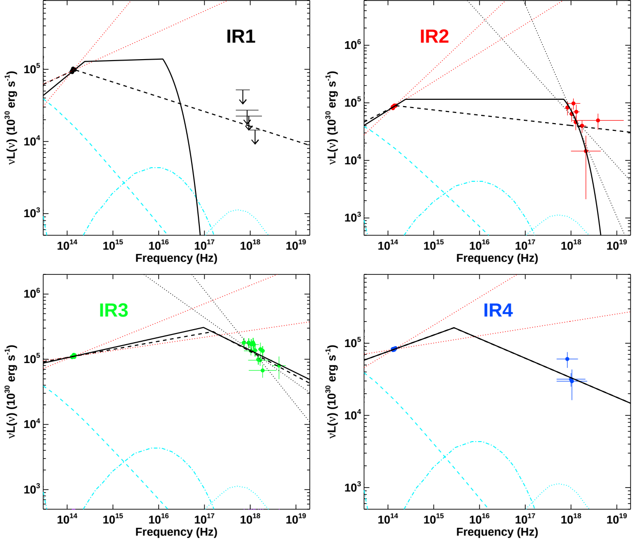
Figure 7. Evolution of Sgr A*'s SED during the very bright flare VB3. Each panel shows the SINFONI and simultaneous X-ray spectra fitted with the PLCool model, during each of the 4 SINFONI spectra integrated during the VB3 flare (see Fig. 5). The colour code is the same as in Fig. 5, with the temporal sequence: black; red; green and; blue. The red and black dotted lines show the uncertainties in the determination of the NIR and X-ray power-law slopes, respectively. The X-ray slopes are well determined only for the IR2 and IR3 spectra. The black dashed lines show the best fit PLCool models, where \Gamma_X = \Gamma_{NIR} + 0.5 is imposed. For IR2 the observed X-ray slope is inconsistent with the predictions of the PLCool model. For both IR1 and IR2 the cooling break is suspiciously pegged in the NIR band. The black solid lines show the best fit PLCoolEv models. During IR1 both the cooling break and the cut-off have large uncertainties, but are constrained to lie within few 10^{14} < \nu < 10^{18} Hz. During IR2 the cut-off is in the X-ray band. From IR2 to IR3 the cooling break evolves to higher energies and then back to lower energies during IR4. Sgr A* is undetected in X-rays during observation IR1. Such as in Fig. 4 both data and models are de-absorbed and corrected for the effects of the dust scattering halo. For a description of the other lines see Fig. 1.
