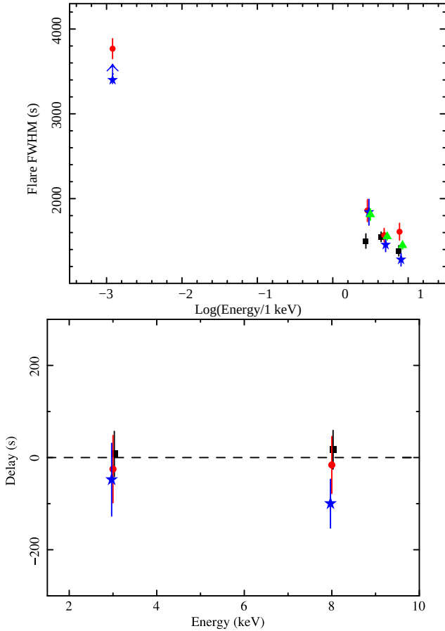
Figure 11. ( Top panel ) Flare duration (FWHM) at various energies of the three brightest XMM-Newton flares, VB1, VB2, VB3 and of the combined XMM-Newton flare light curve are shown with back squares, red circles, blue stars and green triangles, respectively. The flare duration is computed in the 2-4, 4-6 and 6-10 keV energy bands (the points are slightly shifted for display purposes). Flares are typically shorter at higher energies. We also show the duration of VB2 (as observed in the L' band, see §5.2) and the lower limit on the duration of VB3 (as observed with SINFONI ). The flare durations in the NIR band connect with the extension of the trend observed in X-rays. ( Bottom panel ) Peak occurrence delay, between different energies (same energy bands as above) for the three very bright flares observed by XMM-Newton . The delays are computed as the best fit peak value of the Gaussian at each energy minus the same value observed in the 4-6 keV band. Colour code as before.
