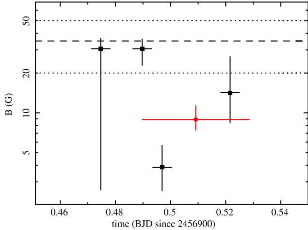
Figure 9. Evolution of the strength of the magnetic field (in Gauss) during and after the flare VB3, in the PLCoolEv model. The black square show the magnetic field strength during IR1 to IR4. The red circle shows the measurement of the average magnetic field during the entire duration of the X-ray flare VB3 (under the assumption of a constant escape time of t_{esc} = 300 s). The dotted lines indicate the typical range of magnetic field strengths during quiescence ( B \sim 20 - 50 G). The dashed line shows the magnetic field strength ( B \sim 36 G) corresponding to a cooling break within the narrow SINFONI band. The flat NIR slopes observed at all times during the flare suggest B < 36 G, while the steep NIR slope observed after the VB3 flare (during IR5, IR6 and IR7) suggest B > 36 G. The error bars correspond to the 1-sigma uncertainties as derived from the confidence contours shown in Fig. 8. No evidence for a cut off at or below the X-ray band is observed during IR4, therefore the associated measurement is valid under the assumption that the cut off is at energies higher than the X-ray band. Would this assumption be invalid, such constraint should be considered as a upper limit.
