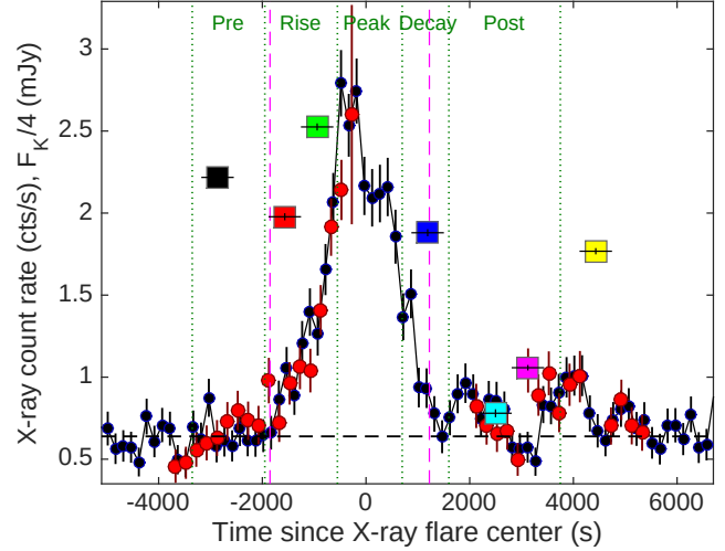
Figure 5. The black and red points show the XMM-Newton 2–10 keV (sum of the three EPIC cameras) and NuSTAR 3–20 keV light curve of Sgr A*’s flare VB3 (Ponti et al. 2015). A constant rate of 0.13 \text{ cts s}^{-1} has been subtracted from the NuSTAR light curve for display purposes, to take into account the different contribution of the diffuse and quiescent emission (gaps in the NuSTAR light curve are due to Earth occultation). The squares show the extinction corrected SINFONI light curve of Sgr A* during the VB3 flare. Each point corresponds to a NIR spectrum integration time of 600 s. The y-axis reports the observed renormalised (divided by 4 for display purposes) flux density at 2.2 \mu\text{m} in mJy units. The black dashed line indicates the level of the “non-flare” (quiescent in X-rays) emission. The pink dashed lines indicate the start and end of the XMM-Newton VB3 flare, as indicated by the Bayesian block decomposition (see Ponti et al. 2015a). Excess X-ray emission is observed \sim 2000 and \sim 4000 s after the X-ray flare peak. The dotted green lines show the intervals for the integration of the pre-, rise, peak, decrease and post-flare spectra during VB3. The zero point of the abscissa corresponds to 525831144.7 s ( \text{TT}_{\text{TBD}} ) and 2456900.50784 day ( \text{BJD}_{\text{TBD}} ), respectively.
