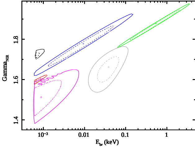
Figure 8. The black, red, green, blue and grey lines show confidence contours of the uncertainty on E_{br} and \Gamma_{NIR} for IR1, IR2, IR3, IR4 and the mean spectrum once fitted with the PLCool model, respectively. The dotted and solid lines show the 68 and 90 % confidence contours, respectively. During IR1 and IR2 the cooling break pegs at its lowest value, being located just above the NIR band. Once fitted with the PLCoolEv model, the confidence contours remain unchanged for IR3, IR4 and the mean spectrum, because during these intervals the high energy cut off is at very high energy. The magenta lines show the confidence contours during IR2, when the cut off is observed in the X-ray band. During IR1, the cut off falls between the NIR and X-ray band, therefore the location of the cooling break is unconstrained.
