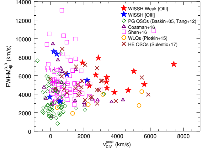
Fig. 9. \text{FWHM}_{\text{Hg}}^{\text{BLR}} as a function of v_{\text{CIV}}^{\text{peak}} for the WISSH sample, compared to PG QSOs from Baskin & Laor (2005) and Tang et al. (2012) (green diamonds), WLQs from Plotkin et al. (2015) (orange circles), SDSS QSOs from Shen (2016) and Coatman et al. (2016) (magenta squares and purple triangles, respectively) and HE QSOs from Sulentic et al. (2017).
