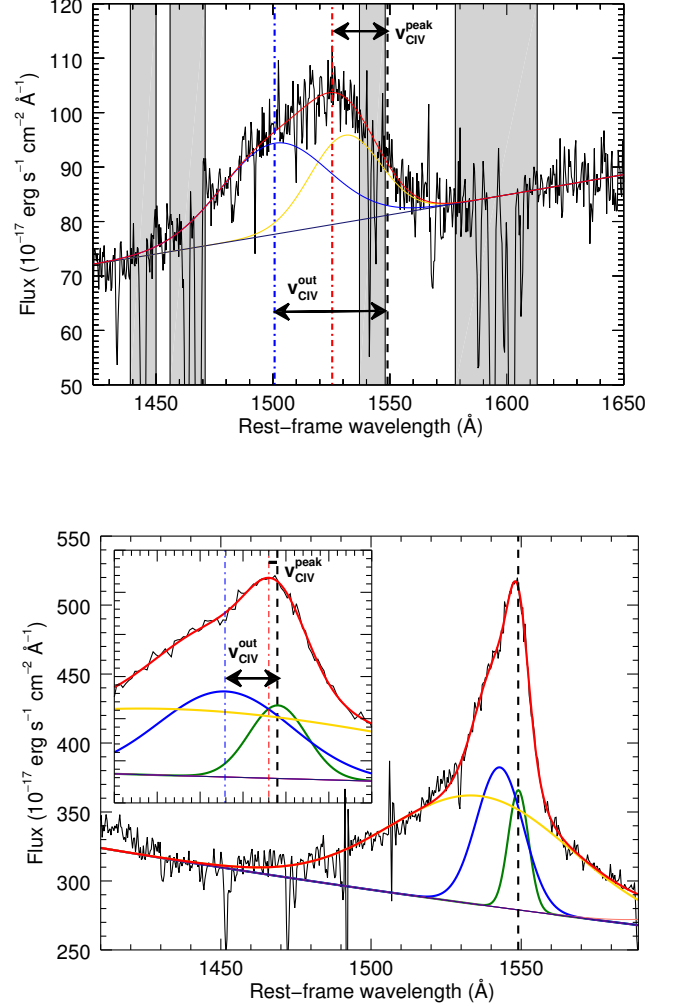
Fig. 2. Parametrization of the CIV emission line profile of the Weak [OIII] quasar J1422+4417 (Upper panel) and the [\text{OIII}] quasar J0745+4734 (lower panel). In both panels the red, yellow and blue curves refer to the best-fit of the spectrum, virialized component and outflow component of the CIV emission line, respectively. The black dashed line indicates the \lambda_{\text{CIV}} at 1549 Å. The red dotted-dashed line denotes the peak of the CIV emission line and v_{\text{CIV}}^{\text{peak}} represent its velocity shift with respect to the systemic \lambda 1549 Å. The blue dotted-dashed line indicates the peak of the outflow component and v_{\text{CIV}}^{\text{out}} is its velocity shift with respect to the systemic redshift. In the lower panel the green curve refers to an additional Gaussian component required by the fit, in order to better described the CIV profile in this QSO.
