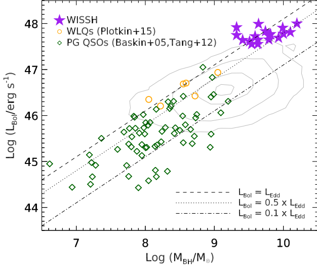
Fig. 5. Bolometric luminosity as a function of BH mass for the WISSH sample, compared to PG QSOs from Tang et al. (2012) and Baskin & Laor (2005) and WLQs from Plotkin et al. (2015). Luminosity in fractions of 0.1, 0.5 and 1 Eddington luminosity are respectively indicated with dot-dashed, dotted and dashed lines. Contours levels (0.01, 0.1, 0.5, and 0.9 relative to the peak) refer to SDSS DR7 QSOs from Shen et al. (2011).
