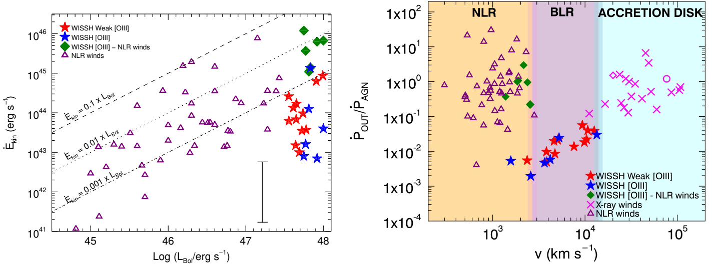
Fig. 11. (left) Kinetic power of the CIV outflow component as a function of L_{\text{Bol}} for the WISSH QSOs (red and blue stars) compared with WISSH NLR ionized outflows from Paper I (green diamonds) and other samples from literature, (e.g. Fiore et al. 2017 for details) (purple triangles). The error bar (bottom right corner) is calculated as described in Sect. 4.3.2. (right) Wind momentum load as a function of the outflow velocity. The BLR winds traced by the CIV outflow components from the WISSH QSOs (red and blue stars) are compared with X-ray winds (magenta crosses) and Ionized winds (green triangle). X-ray winds for Markarian 231 and IRAS F11119+13257 are represented with magenta diamond and circle, respectively.
