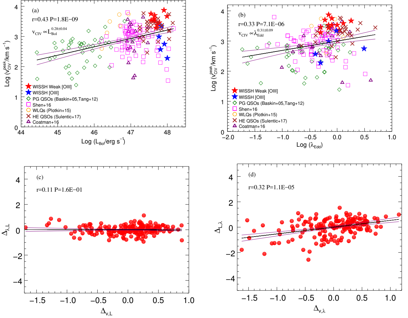
Fig. 12. v_{\text{CIV}}^{\text{peak}} as a function of L_{\text{Bol}} (a) and as a function of \lambda_{\text{Edd}} (b), for the WISSH sample (blue/red stars) compared to the PG QSOs from Baskin & Laor (2005) and Tang et al. (2012) (green diamonds), WLQs from Plotkin et al. (2015) (orange circles) and SDSS QSOs from Shen (2016) and Coatman et al. (2016) (magenta squares and purple triangles) and HE QSOs from Sulentic et al. (2017, and reference therein). The L_{\text{Bol}} for the HE sample has been derived from L_{5100} applying a bolometric correction of 5.6, as suggested by Runnoe et al. (2012) for the luminosity range of the HE sample. (c) Residuals plot of \lambda_{\text{Edd}} - L_{\text{Bol}} and v_{\text{CIV}}^{\text{peak}} - L_{\text{Bol}} relations. (d) Residuals plot of L_{\text{Bol}} - \lambda_{\text{Edd}} and v_{\text{CIV}}^{\text{peak}} - \lambda_{\text{Edd}} relations. The black lines indicate the best linear fits to the data and the purple lines correspond to the 68% confidence interval.
