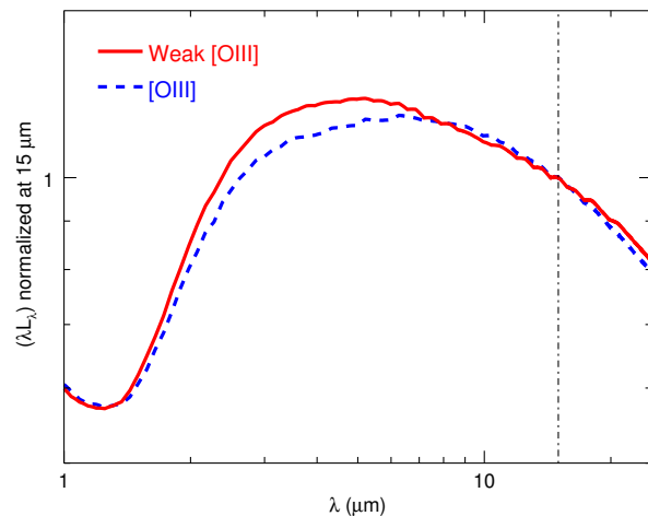
Fig. 4. Average SEDs corresponding to WISE photometry of the WISSH [OIII] (dashed blue line) and Weak [OIII] samples (red line), normalized at 15\mu m (dot-dashed line).
