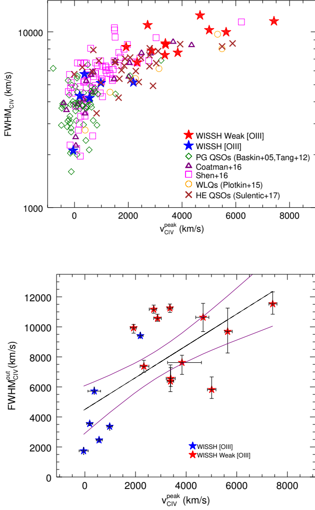
Fig. 8. \text{FWHM}_{\text{CIV}} of the entire emission line profile as a function of v_{\text{CIV}}^{\text{peak}} for the WISSH sample, compared to PG QSOs from Baskin & Laor (2005) and Tang et al. (2012) (green diamonds), WLQs from Plotkin et al. (2015) (orange circles), SDSS QSOs from Shen (2016) and Coatman et al. (2016) (magenta squares and purple triangles respectively) and HE QSOs from Sulentic et al. (2017) ( top ) and \text{FWHM}_{\text{CIV}}^{\text{out}} of the outflow component ( bottom ), as a function of v_{\text{CIV}}^{\text{peak}} for the WISSH sample. The black solid line indicates the best linear fits to the data and the purple dashed lines correspond to the 68% confidence interval.
