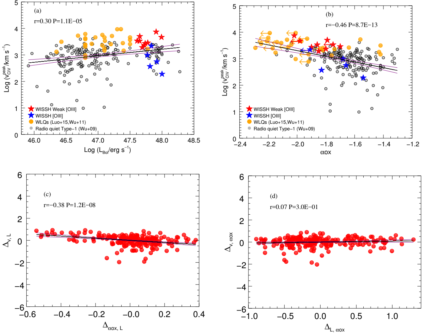
Fig. 13. v_{\text{CIV}}^{\text{peak}} as a function of L_{\text{Bol}} (a) and \alpha_{\text{OX}} (b), for the WISSH sample (blue/red stars) compared to Radio quiet Type-1 QSOs from Wu et al. (2009) (black circles) and WLQs from Wu et al. (2011) and Luo et al. (2015) (orange circles). (c) Residuals plot of v_{\text{CIV}}^{\text{peak}} - L_{\text{Bol}} and \alpha_{\text{OX}} - L_{\text{Bol}} relations. (d) Residuals plot of v_{\text{CIV}}^{\text{peak}} - \alpha_{\text{OX}} and L_{\text{Bol}} - \alpha_{\text{OX}} relations. The black lines represent the best linear fits to the data and the purple lines correspond to the 68% confidence interval.
