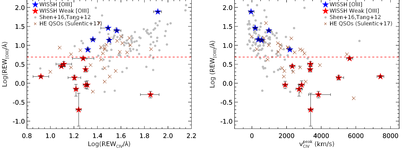
Fig. 7. Rest-frame EW of [OIII]λ5007 as a function of REW CIV ( left ) and v_{\text{CIV}}^{\text{peak}} ( right ) for the WISSH targets with blue stars for the [OIII] sample and red stars for the Weak [OIII] sample, compared to the Shen (2016), Tang et al. (2012) and Sulentic et al. (2017, and reference therein). The dashed red line refers to the WISSH [OIII] dichotomy, with REW [OIII] boundary value of 5 Å.
