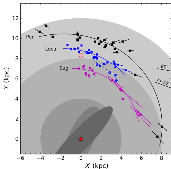
Fig. 2. Location of HMSFRs determined by trigonometric parallax.
