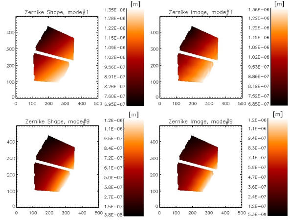
Fig. 9. Result of the Zernike test for modes 1 and 9: comparison between analytical shape (left) and actual result on the M4DP.
