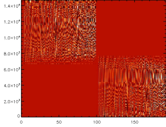
Fig. 3. Optical interaction matrix M of the M4DP: each columns contains the pixel values of a phasemap representing a mirror mode.
