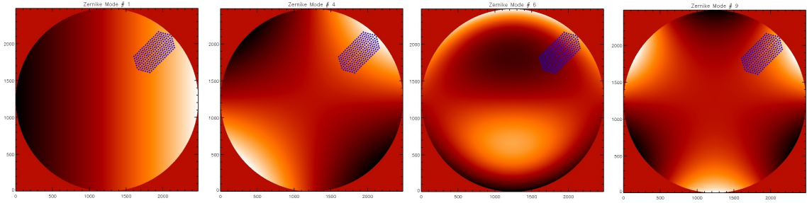
Fig. 5. Zernike shapes cropped according to the DP geometry on M4.
