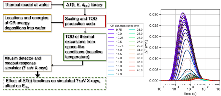
Fig. 6 Left: Simulation workflow, showing the evolution from thermal model to simulated TOD and energy resolution impact estimations. Right, solid lines: 500 keV simulated pulses; Right, black dashed lines: 50 MeV pulses, downscaled to 500 keV; Right, dashed red lines: Half-distance scaled and energy-scaled 50 MeV pulses. (Colour figure online)
