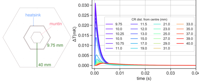
Fig. 4 Results of the thermal model, for a 500 keV heat pulse at locations varying between 9.75 to 40 mm from the central-most pixel (0,0). Left: Diagram of the wafer, showing the location of the pixel and muntin regions, heatsink, and representation of varying CR injection distances (green line). (Colour figure online.)
