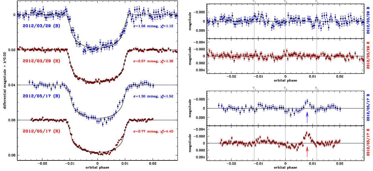
Fig. 1. Left panel: light curves of GJ1214b gathered through the blue channel of LBC in the Bessel B band (blue points), and through the red channel in Bessel R (red points). Data points are plotted with the original sampling cadence. The black line corresponds to the best-fit model adopting the parameters listed in Table 2. Right panel: same as above, but showing the residuals from the best-fit model. The bump-like feature at phase 0.070 \lesssim \phi \lesssim 0.092 appeared during the second transit and is interpreted as a starspot crossing; it is marked with an arrow in both channels.
