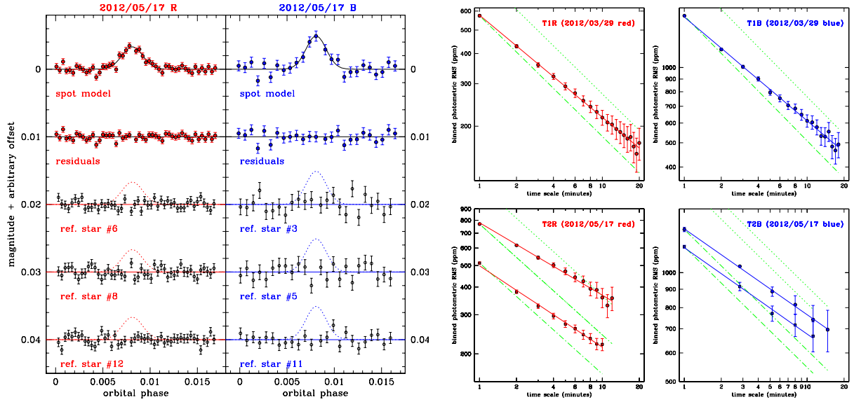
Fig. 3. Left panel: modeling of the T2/R (left plots) and T2/B (right plots) light-curve bumps. From the top: residual light curves with the best-fit Gaussian model overlaid (black line; Table 1), residuals from the Gaussian fit, and light curves of three reference stars with a red color and magnitude similar to GJ1214. Within the errors, the bump-like feature is not seen in any other light curve. Right panel: correlated noise diagrams (photometric RMS of the binned time series as a function of bin size) for the GJ1214b LBC residual light curves after the best-fit transit model has been subtracted. The lower sequence in the T2/B, T2/R plots is evaluated after the starspot feature has been masked out. The green lines follow a Poisson-like 1/\sqrt{N} scaling law as extrapolated from the RMS of the unbinned curve (dotted-dashed line), and with a 50% increase as reference (dotted line).
