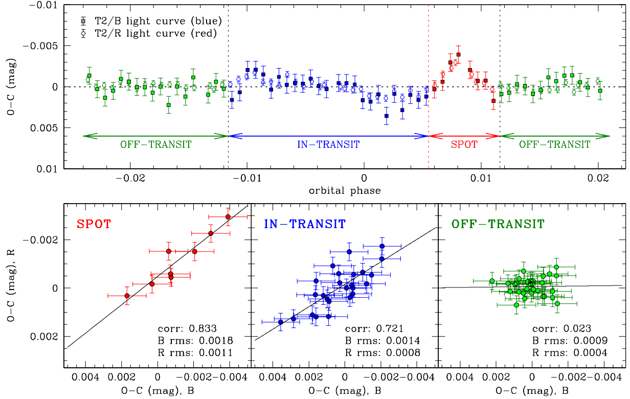
Fig. 4. Statistical correlation between the blue (T2/B) and red (T2/R) LBC light curve of the second transit. Upper panel: observed minus calculated (O – C) residuals from the best-fit transit model as a function of orbital phase for the T2/B (square points) and the T2/R (round points) time series. Data are color-coded according to whether they are labeled as off-transit, in-transit (the spot feature being excluded) and spot only. Only points whose mid-exposure time can be matched within 30 s to a frame of the other channel are considered here. Lower panels: correlation plots between residuals from T2/B and T2/R light curves for the three samples defined above. The best-fit straight line calculated by ordinary least-squares is overplotted. The Spearman rank correlation coefficient is tabulated for each subset, along with the blue and red RMS.
