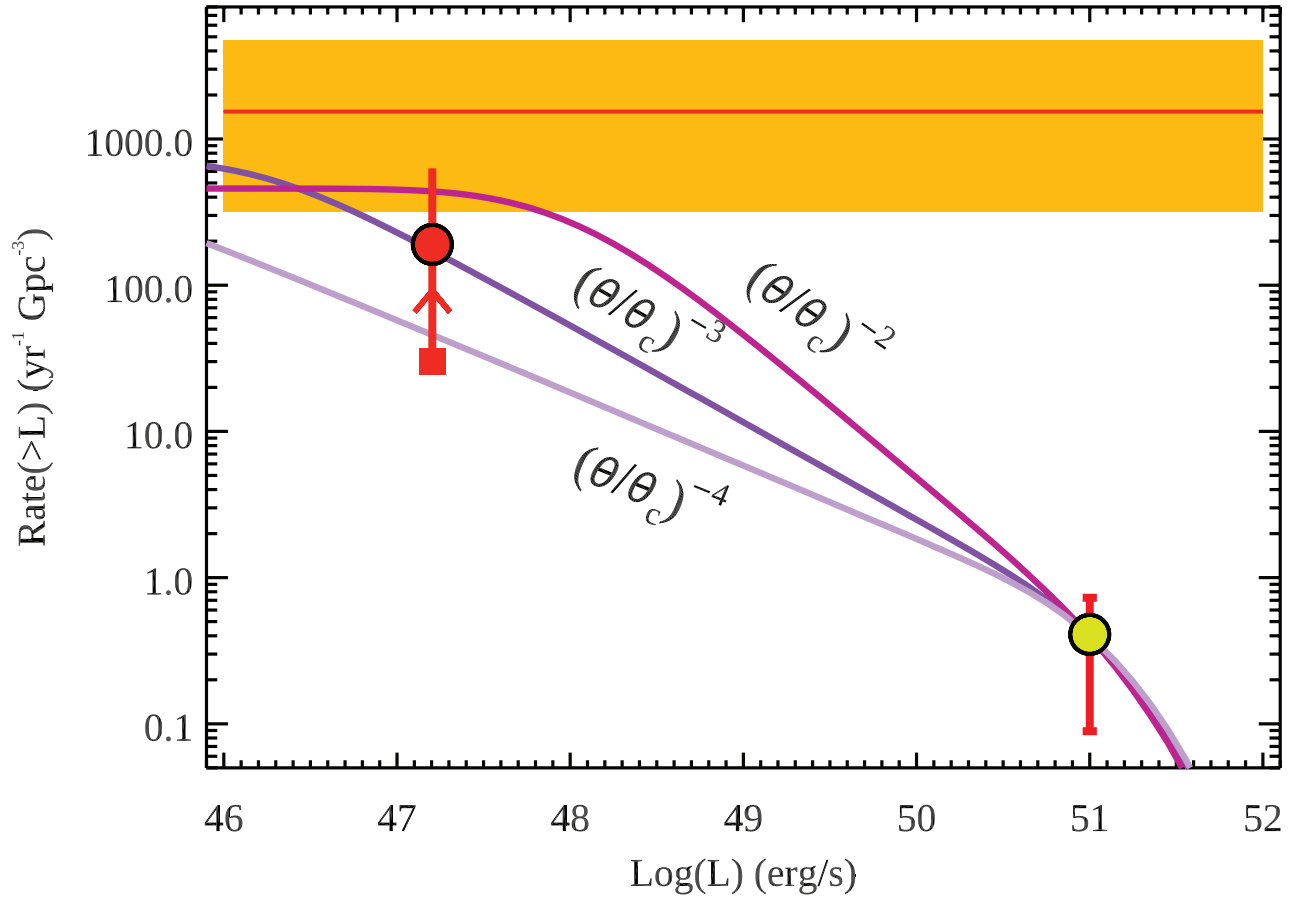
Fig. 4. Short GRB rate as a function of luminosity. The rate of short GRBs with isotropic equivalent luminosity L_{\text{iso}} > 10^{51} \text{ erg s}^{-1} (yellow filled symbol - 27) is compared with the expected rate of short GRBs similar to GRB 170817A (solid red symbol (34)). We consider this a lower limit: GRB170817A, detected by the Fermi spacecraft, is the only one of its class with an associated GW event, but Fermi could have detected similarly dim events without an associated GW event. Lines show predictions for different jet structures, consistent with the estimate based on the detected luminosity of GRB 170817A. The solid red horizontal line (the orange shaded region is its 1\sigma uncertainty) shows the rate of binary neutron stars (BNS) mergers inferred from GW data alone (1).
