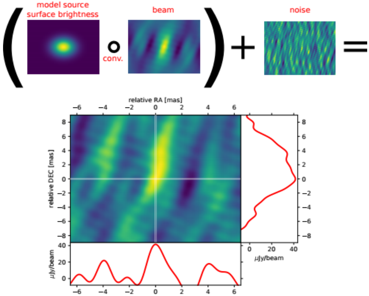
Figure S5: Depiction of our Monte Carlo posterior probability calculation. To produce the needed peak brightness samples, the model image is convolved to the beam, and a noise realization is added to obtain a simulated source image (an example of which is shown above, along with plots of the brightness distribution along the central axes, highlighted in white), whose peak brightness is recorded. The procedure is repeated for a large number of noise realizations (obtained by placing the convolved source image at random position of the noise image) and for a large number of source total flux densities sampled from the prior. Gaussian kernel density estimation is then used on the produced peak brightness samples to compute the un-normalized, marginalized posterior for each size. Varying the source image size on a grid we obtain the posterior probabilities shown in Figures S3 and S4.
