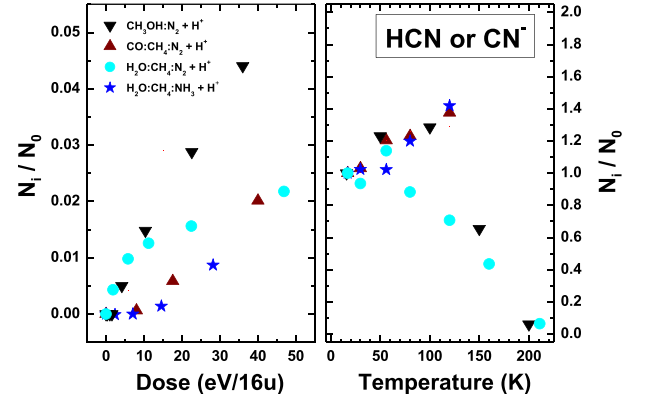
Figure 5. Left-hand panel: normalized HCN/CN - abundance produced after: black down triangles – irradiation of CH 3 OH:N 2 (1:1) ice mixture with 200 keV H + (experiment 1.1); wine up triangles – irradiation of CO:CH 4 :N 2 (1:1:1) ice mixture with 200 keV H + (experiment 2); cyan circles – irradiation of H 2 O:CH 4 :N 2 (1:1:1) ice mixture with 200 keV H + (experiment 4); blue stars – irradiation of H 2 O:CH 4 :NH 3 (1:1:1) ice mixture with 200 keV H + (experiment 5). Irradiation of ice mixtures is carried out at 17 K, with CH 3 OH:N 2 ice irradiation done at 16 K. Normalization is performed to the initial CH 4 or CH 3 OH abundance. Right-hand panel: evolution of HCN/CN - abundance with annealing of the ice. The values are normalized to the final abundance of the species obtained in the experiments showed on the left-hand panel and keep the same labelling.
