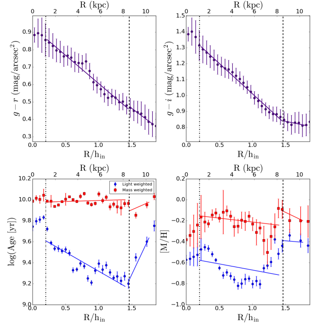
Fig. 3. g-r and g-i colour (top panels) and stellar age and metallicity (bottom panels) profiles for IC 1199 as an example. The colour profiles are represented by means of purple circles (top panels). Blue circles represent light-weighted stellar age or metallicity; red squares symbolise mass-weighted stellar age or metallicity (bottom panels). The dot-dashed vertical line delimits the bulge-dominated region ( R_{\text{lim},\text{in}} ), while the dashed vertical is located at the break radius ( R_{\text{break}} ).
