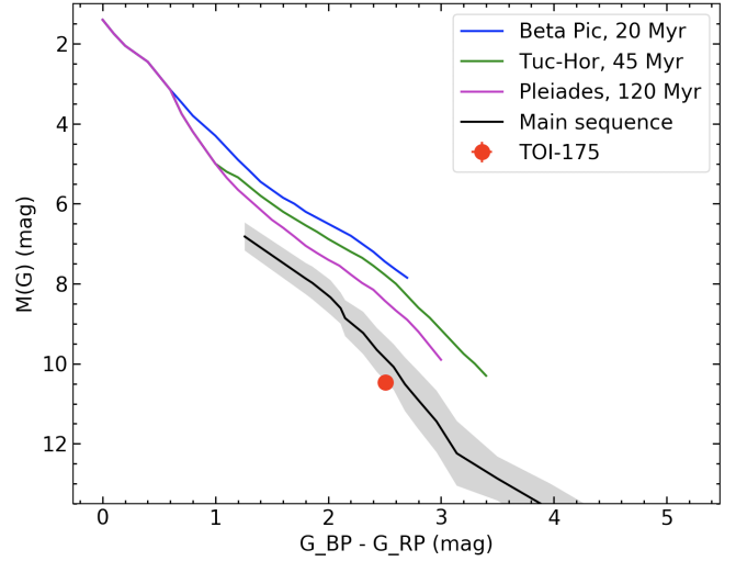
Fig. 1. Absolute magnitude (in the G Gaia bandpass) vs. color (magnitude difference between the Gaia bands G_{\text{BP}} and G_{\text{RP}} ): L 98-59 A (TOI-175) is located in the Gaia color-magnitude diagram together with the mean sequences of young clusters and moving groups (Luhman 2018) and the main sequence of stars (Cifuentes et al. 2020). The error bars of L 98-59 A are smaller than the symbol size. The gray area represents the 1\sigma dispersion of field M dwarfs.
