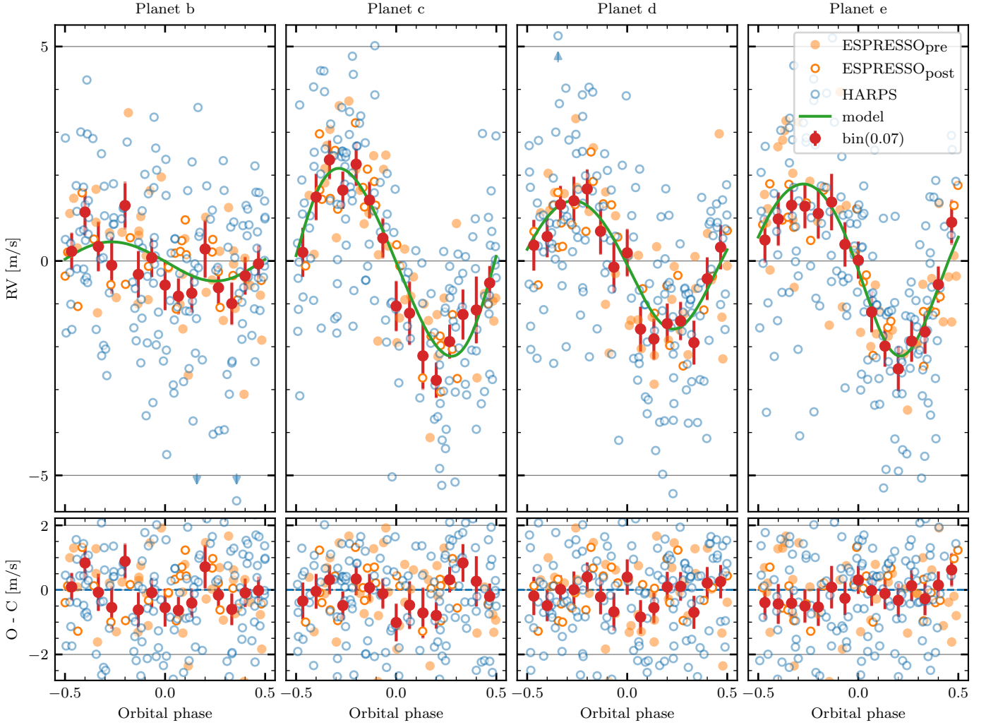
Fig. 6. Phase-folded HARPS and ESPRESSO RVs, best model ( top ) and residuals ( bottom ) for the four planets. The HARPS data, presented in Sect. 2.1.1, are displayed with empty blue circles, and the ESPRESSO data, presented in Sect. 2.1.2, are displayed with orange circles. The filled orange circles are for the data taken before the fiber change of ESPRESSO. The empty orange circles are for data taken after the change. For clarity, the error bars of the HARPS and ESPRESSO data points are not displayed. For this plot, the stellar activity model has been subtracted from each data point. The points with error bars in red correspond to averages of the data within evenly spaced bins in orbital phase, whose size is 0.07 orbital period. The best model is shown with a green line. Before the subtraction of the stellar activity model the RMS of the RV data is 3.5, 3.4, and 3.2 m s -1 for HARPS, ESPRESSO pre , and ESPRESSO post , respectively. After the subtraction of the stellar activity model, it is 2.9, 2.5, and 2.3 m s -1 for HARPS, ESPRESSO pre , and ESPRESSO post , respectively. Finally, after subtraction of the planetary model, the RMS of the residuals is 1.8, 1.2, and 0.7 m s -1 for HARPS, ESPRESSO pre , and ESPRESSO post , respectively.
