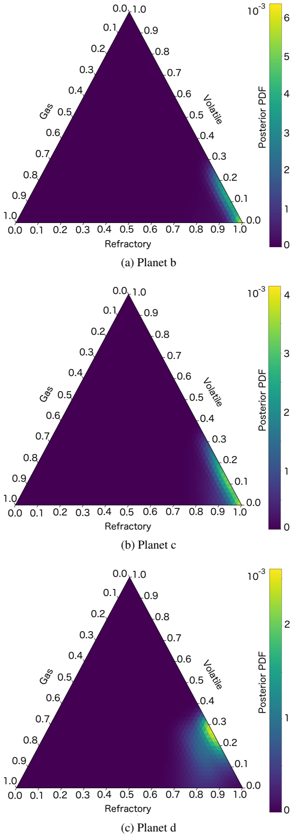
Fig. 9. Ternary diagrams showing the internal composition (mass fractions of the gas (H and He), the volatile (water) and the refractory elements) for the three transiting planets in system L 98-59.
