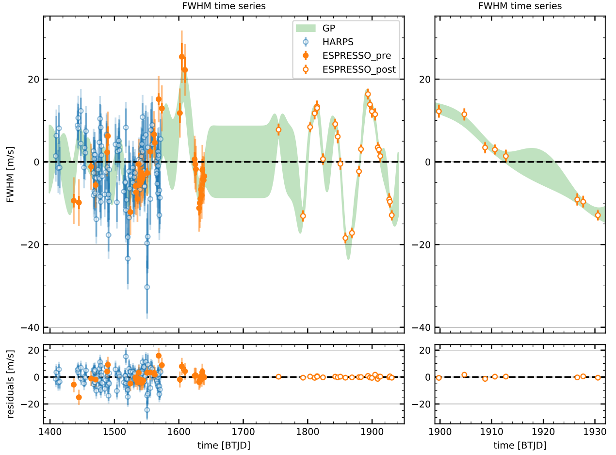
Fig. F.3. Outcome of the fit of the four-planet model regarding the FWHM: The structure of this figure is similar to that of Fig. 4 or Fig. F.1 , but the FWHM data and model are displayed instead of the RV data and model.
