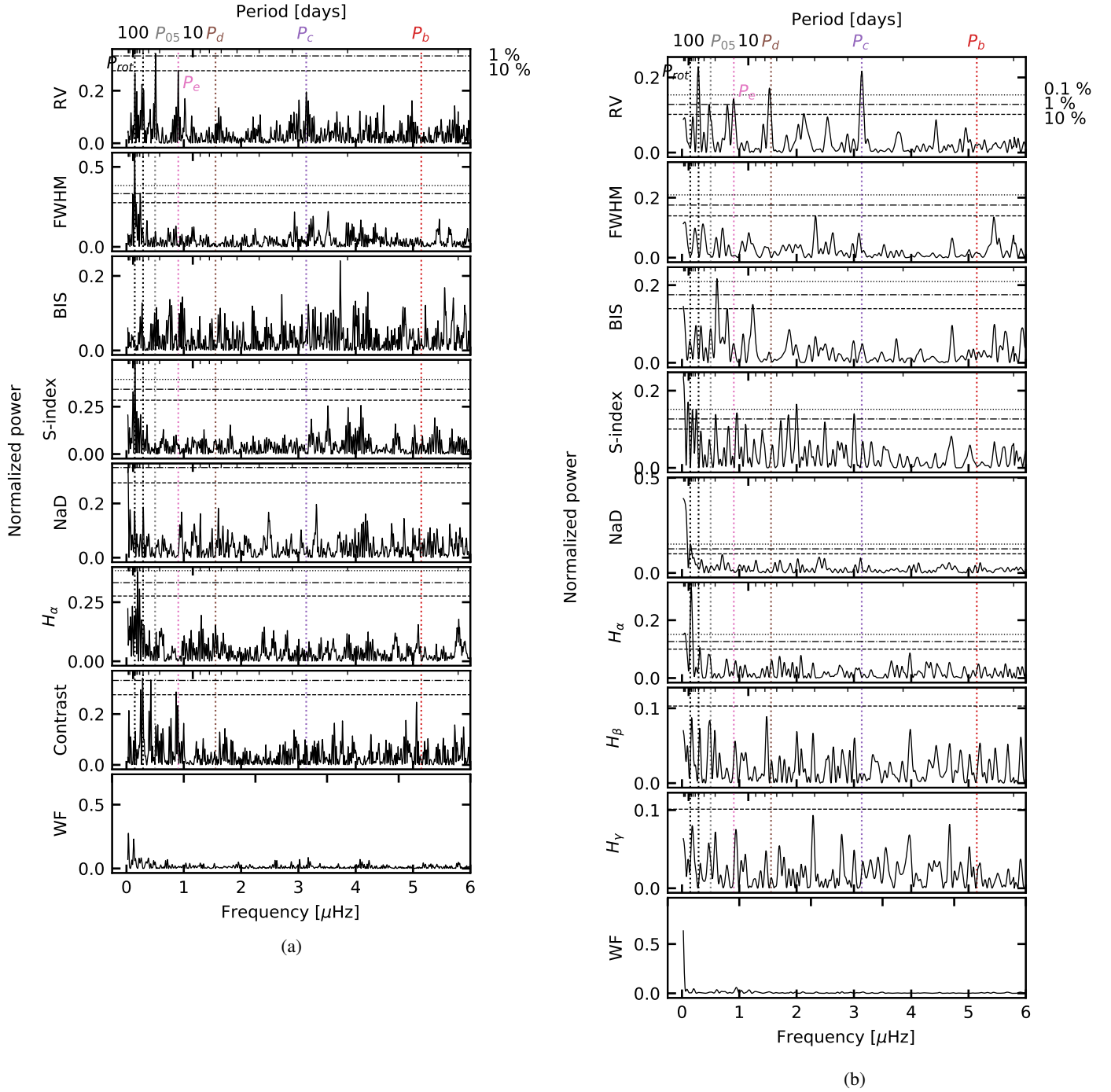
Fig. 2. GLSP of the RV and activity indicators from ESPRESSO (a) and HARPS (b) data. The last row for both instruments presents the window function. The vertical dotted lines indicate from right to left the orbital period of the planets b, c, d, and e, the planetary candidate 05, and half and the full stellar rotation period (assumed here to be 80 days). The horizontal lines indicate the amplitude levels corresponding to 10% (dashed line), 1% (dot-dashed line) and 0.1% (dotted line) of the FAP. The amplitudes of the GLSPs are expressed using the ZK normalization described in Zechmeister & Kürster (2009, Eq. (5)). The FAP levels are computed using the analytical relation also described in Zechmeister & Kürster (2009) for this normalization. We display the GLSP of the BIS for completeness and comparison with C19, but we caution that the reliability of BIS measurements from CCFs for M dwarfs is uncertain (Rainer et al. 2020).
