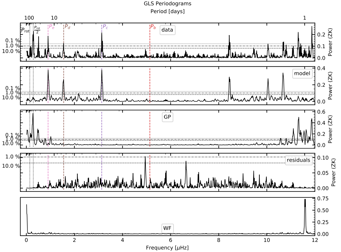
Fig. 5. Outcome of the fit of the four-planet model: GLSPs of the RV time series ( top ) and of the planetary ( second ) and stellar activity ( third ) models sampled at the same time as the RV data, GLSP of the time series of the residuals ( fourth ) and the window function ( bottom ). The vertical lines on the GLSPs correspond to the orbital periods of planets b, c, d, and e, half and the full rotation period (estimated at 80 days) from right to left.
