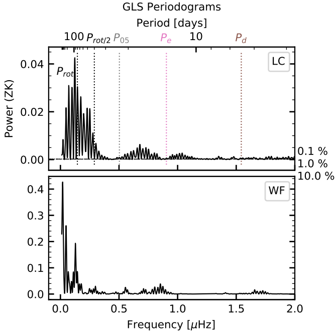
Fig. 3. GLSP of the TESS LC. The format of this figure is identical to that in Fig. 2. In particular, the power of the GLSP is normalized using the ZK normalization. The highest peak in this periodogram is for a period of 93 days.
