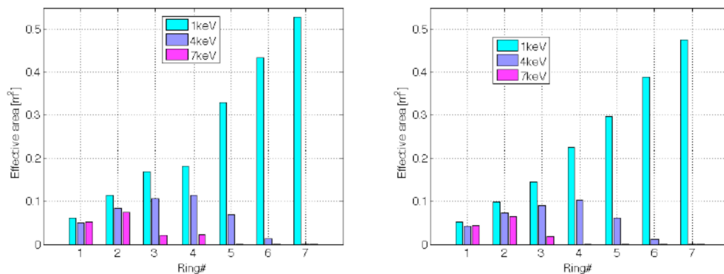
Figure 13 – effective area as function of the energy and diameter
