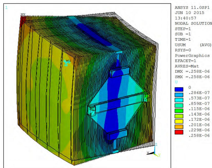
Figure 15 - Displacement [m] under radial temperature gradient (1°C) for the case with parabolic and hyperbolic surfaces slumped together
