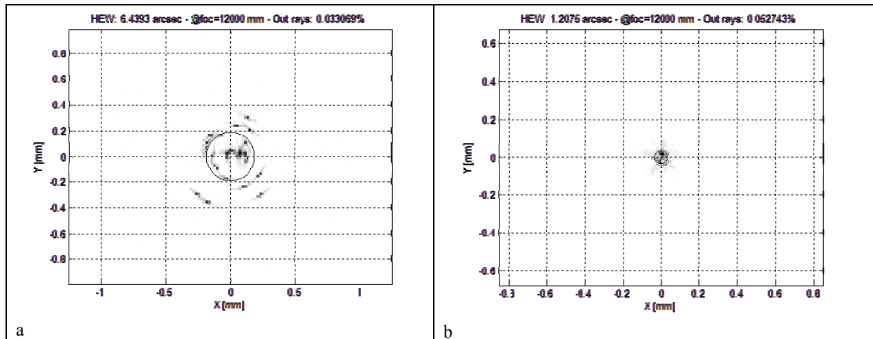
Figure 6 – PSF due to the petal distortion under lateral gravity (for simplicity only ring 5 is considered). HEW intrinsic contribution of each MM of 0.5". 3 points (a) and 6 bipods (b) cases.
