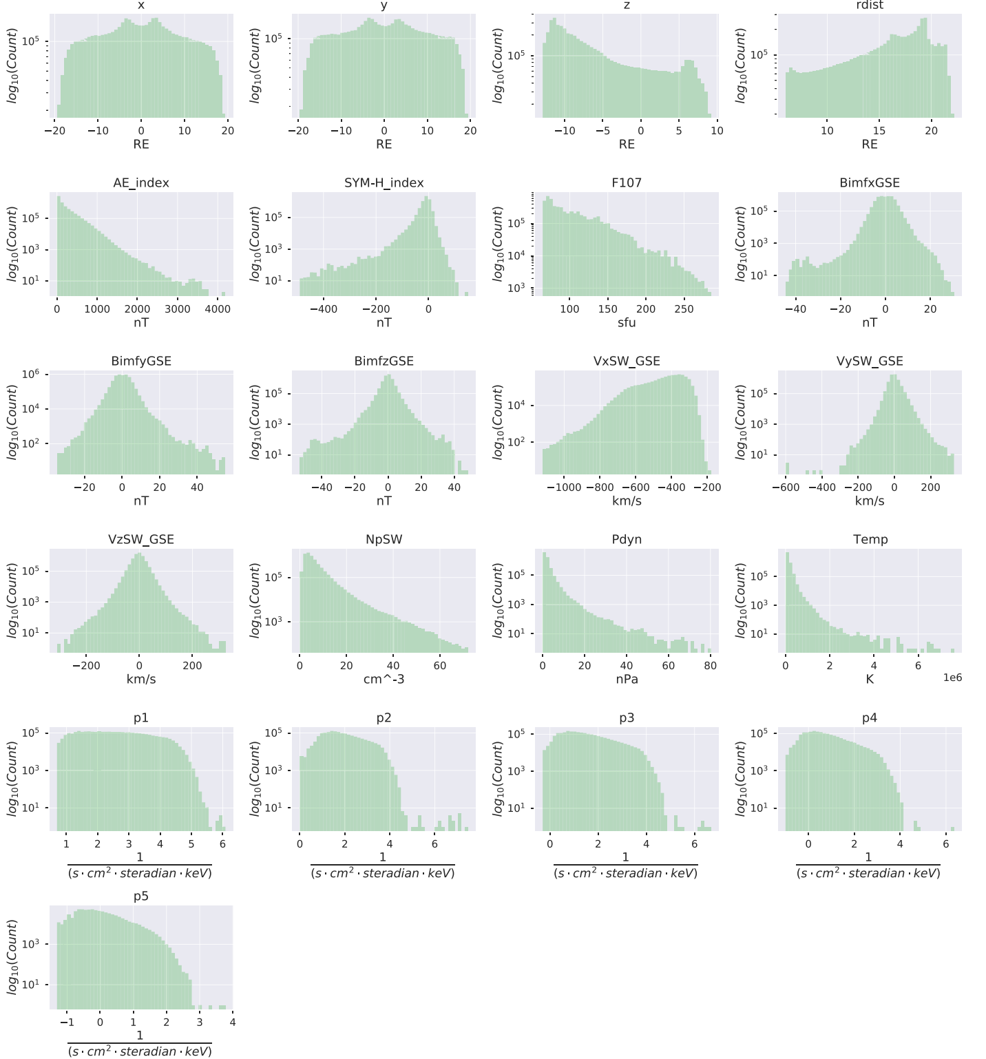
Figure 9. Histogram of the number of samples of predictors and proton intensities used in the model. The intensities per channel are in \log_{10} space.
