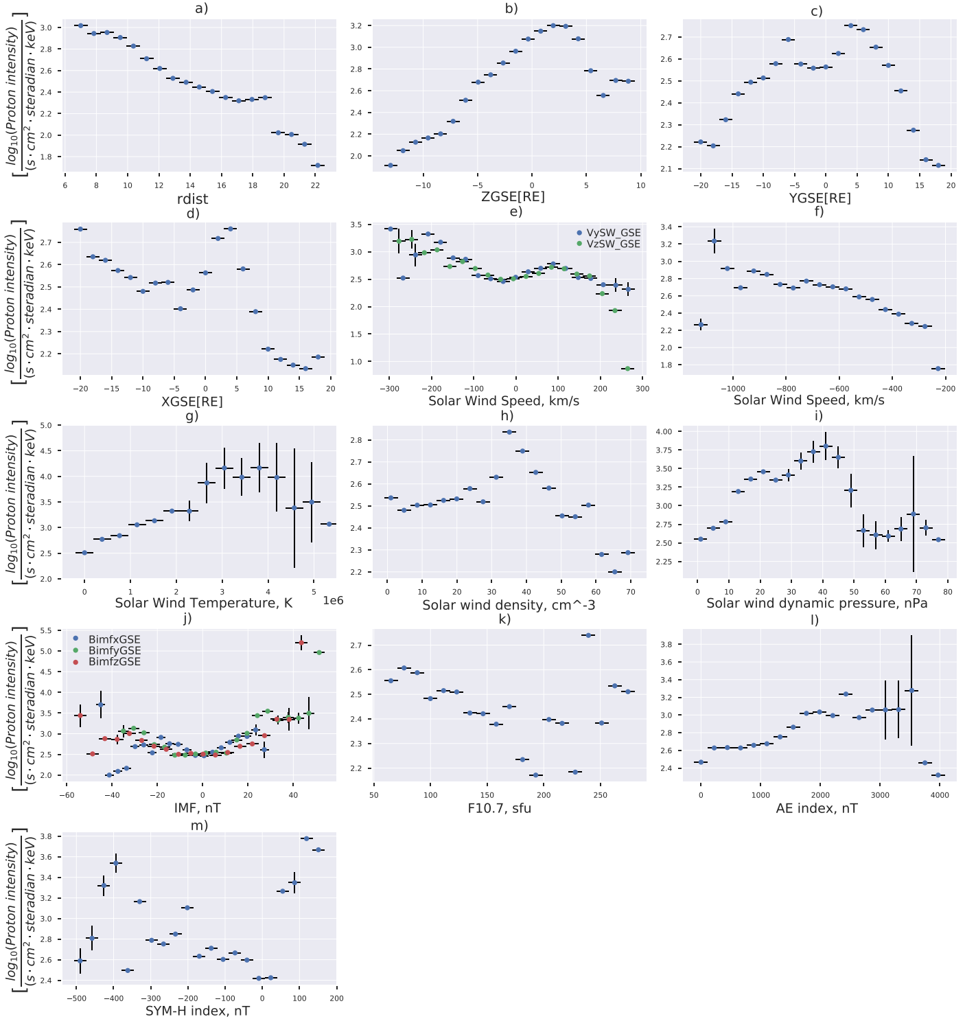
Figure 3. Relations of mean proton intensities for the energy channel 1 and (a)–(d) radial distance, r_{\text{dist}} , ZGSE, YGSE, and XGSE, respectively; (e) the solar wind V_y and V_z components; (f) the solar wind radial velocity, V_r ; (g)–(i) solar wind temperature, density, and dynamic pressure, respectively; (j) IMF components in GSE; (k) F10.7 parameter; (l) AE index and (m) SYM-H index. Vertical lines represent confidence intervals at 95% confidence level. Here zero values of proton intensity are replaced with small values.
