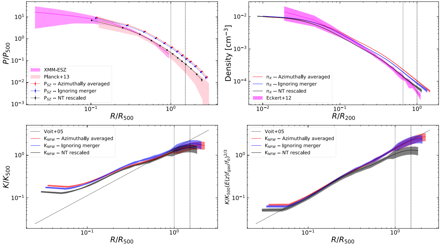
Fig. 17. Rescaled pressure (top left) and density (top right) profiles considering the azimuthally averaged, ignoring the merger, and ignoring the merging region and considering the M_{200,\text{tot}} and R_{200,\text{tot}} required to recover the cosmological gas fraction at the virial radius. We compare these profiles with the Planck envelope (Planck Collaboration Int. V 2013) for pressure, and with the universal density profile (Eckert et al. 2012) for density. Bottom: rescaled entropy and rescaled entropy corrected by the gas mass fraction, before and after correcting for the true total mass.
