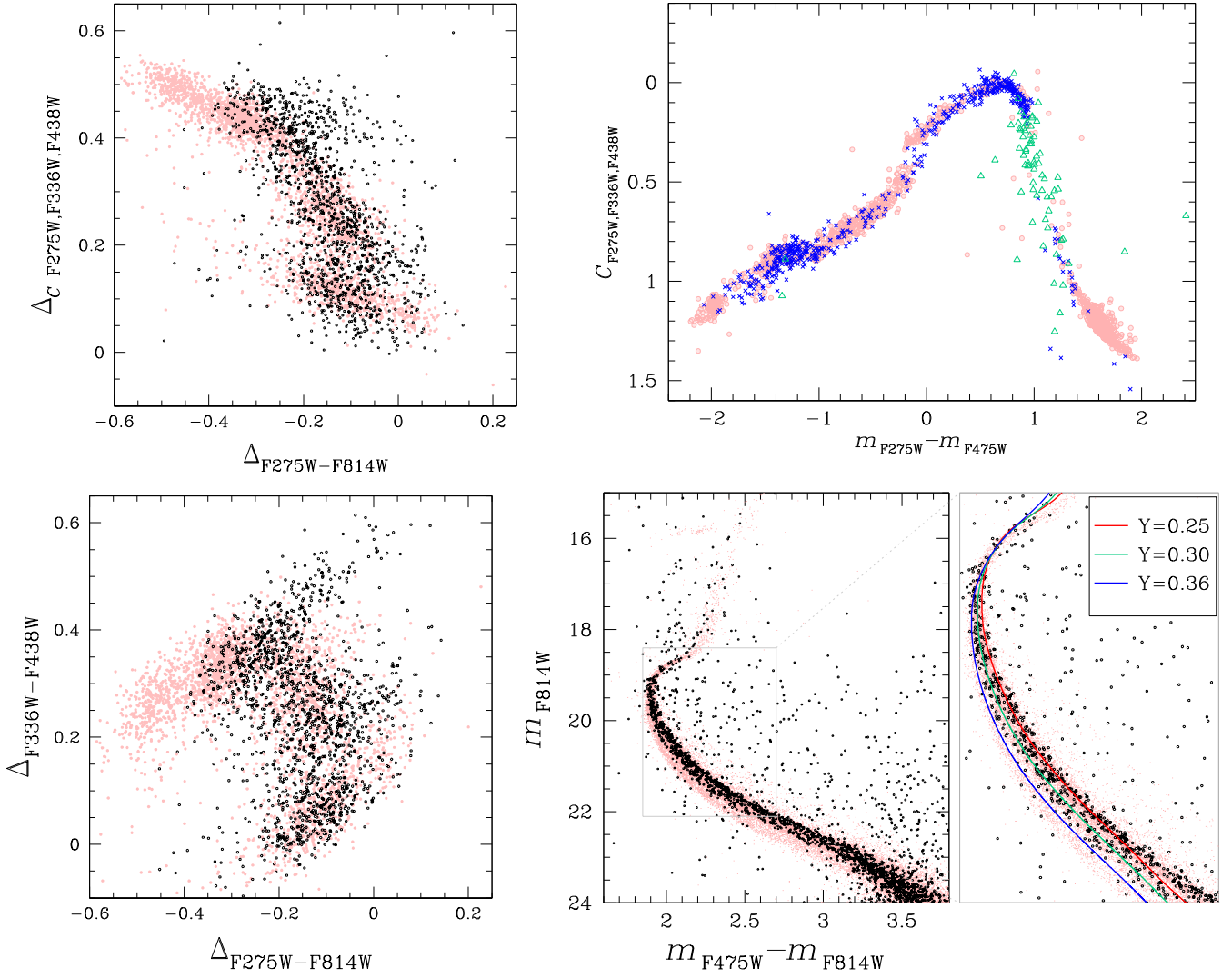
Figure 11. Upper panels: Comparison of the \Delta_{C\text{F275W,F336W,F438W}} vs. \Delta_{F275W-F814W} (upper left) and \Delta_{F336W-F438W} vs. \Delta_{F275W-F814W} ChMs (lower left) of NGC 2808 (pink points) and NGC 6402 (black points). The right panels compare the HBs of NGC 2808 (pink) and NGC 6402 (same colors as in Figure 1; top) and the m_{F814W} vs. m_{F475W} - m_{F814W} CMDs (bottom). We also provide a zoomed-in image of the CMD on the upper MS, where we compare the observations of NGC 2808 and NGC 6402 with isochrones with different helium abundances. See text for details.
