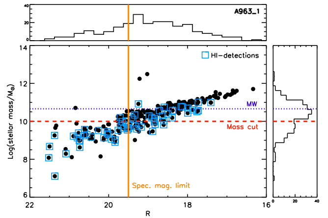
Figure 1. R -band magnitude versus \log(M_*) for the cluster members (black circles). The \text{H I} -detections are distinguished with open blue squares. At the top and right-hand side of the plot, histograms of the R -band magnitude and \log(M_*) are also shown. The dashed red line indicates the mass cut adopted in the analysis of Section 4.3 (see also Section 3), and the dotted blue line is the mass of the MW-like galaxy used as a prototype to explore the effects of ram-pressure stripping in the cluster (cf. Section 4.1). The magnitude limit adopted in the spectroscopic campaign is indicated by the vertical orange line.
