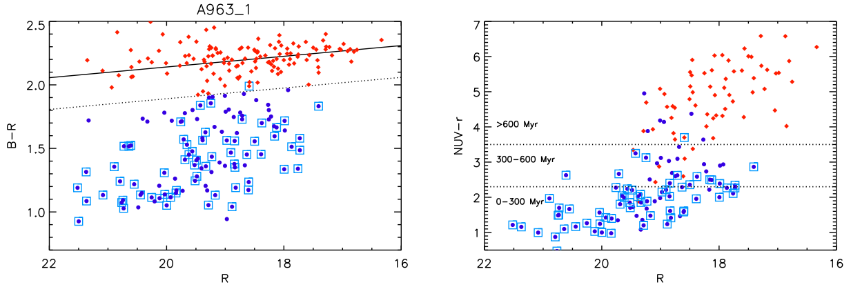
Figure 2. Left: B-R versus R diagram of galaxies in A963_1. The red sequence fit is shown by the solid line. Red-sequence galaxies (red diamonds) are defined to be at most \pm 0.25 mag bluer than the red sequence fit (dotted line). The blue-cloud galaxies (blue circles), are thus located below the dotted line. Right: NUV-optical CMD showing the red-sequence and blue-cloud galaxies defined in the left-hand panel, and dotted lines separating regions (NUV- r colour ranges) that correspond to different stellar-population ages, as labelled (see the text for description). In both panels H I detections are highlighted with open blue squares.
