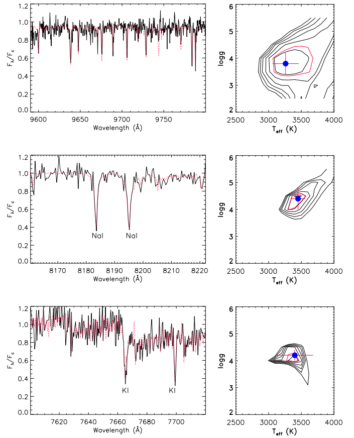
Fig. B.1. Left panels: continuum-normalized VIS X-shooter spectrum of ISO-ChaI 52 in three regions (full black lines) with the best-fitting synthetic spectrum overplotted (dotted red lines). Right panels: \chi^2 contour maps in the T_{\text{eff}} – \log g plane. In each panel, the 1\sigma confidence level is denoted by the red contour. The best values and error bars on T_{\text{eff}} and \log g are also indicated.
