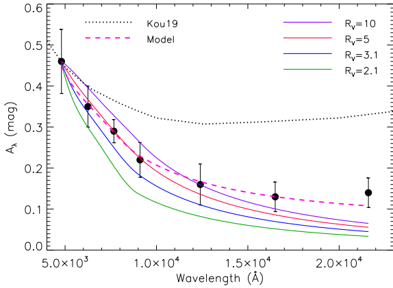
Fig. 3. Extinction taken as the amplitude of the second dip (observed at JD = 2458585) as a function of the filter wavelength (dots). The full lines represent extinction laws at different values of R_V = A_V/E(B - V) according to Cardelli et al. (1989). The dotted black line is the model by Koutoulaki et al. (2019). The dashed line represents our two-component model (Eq. (1)). All curves are normalized to the observed extinction in the g' band ( \lambda_c = 4800 \text{ \AA} ).
