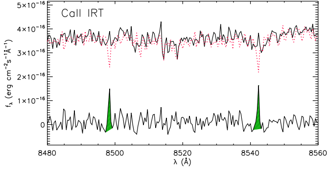
Fig. C.2. X-shooter spectrum of ISO-Chal 52 in the region of Ca II IRT (solid black line) along with the inactive template (dotted red line). The difference between observed and template spectrum is shown in the bottom of the box, along with the residual emission in the line cores (hatched green areas).
