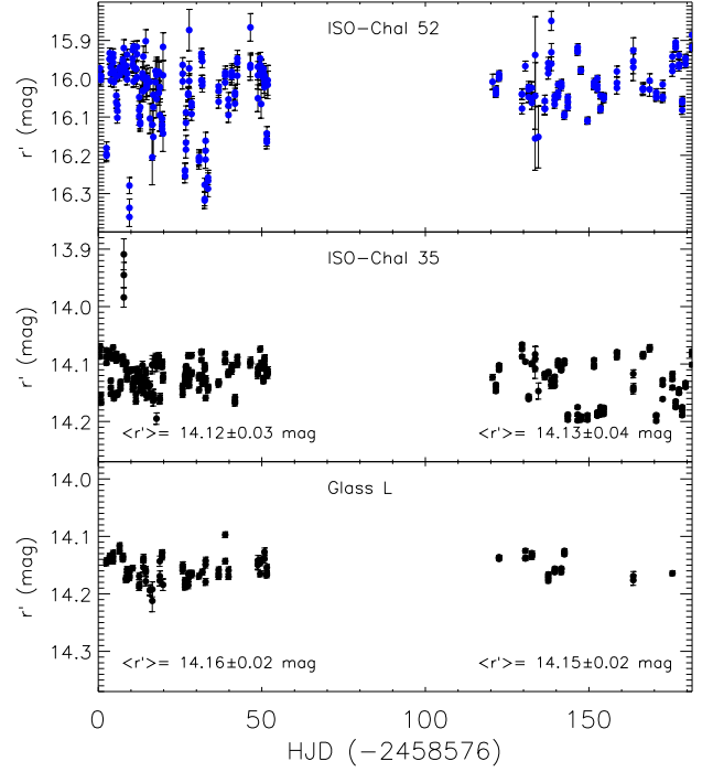
Fig. A.2. ROSS2 r' light curve of ISO-ChaI 52 (top panel), ISO-ChaI 35 (middle panel), and Glass L (bottom panel). We have used 2MASS J11042217–7741319 (star 2) for the first two stars and Glass M (star 5) for the latter as comparison stars, adopting the magnitudes listed in Table A.1. The average magnitudes of the last two stars and their rms scatter are provided in the respective panels for the two data segments.
