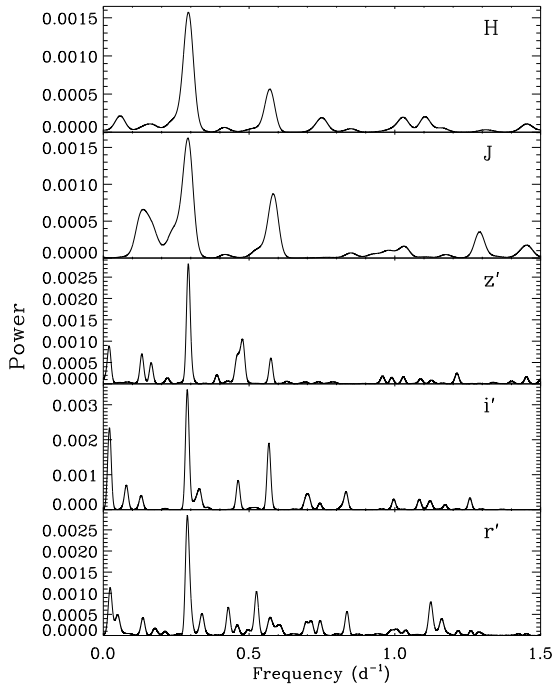
Fig. C.3. Cleaned periodograms for the photometric data of ISO-Chal 52 in the HJz'i'r' bands (from top to bottom). The highest peak in each band corresponds to a period of about 3.45 days.
