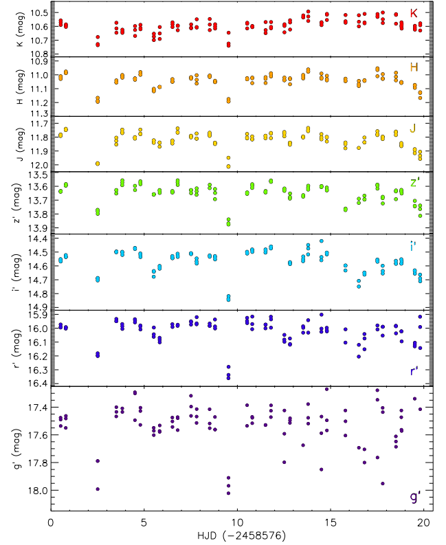
Fig. 2. REM multiband optical/NIR light curves of ISO-Chal 52 for the first 20 days of the campaign. The scales of the vertical axes have been chosen so as to keep the magnitude ranges constant to display the variation amplitudes more clearly.
