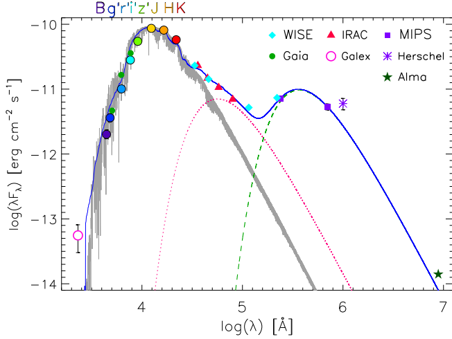
Fig. 1. Spectral energy distribution of ISO-Chal 52. Mid- and far-infrared fluxes are shown with different symbols, as indicated in the legend. The BT-Settl spectrum (Allard et al. 2012) that provides the best fit to the star photosphere is shown by a gray line. The two black bodies with T = 650 K and T = 100 K that fit the MIR and FIR disk emission are shown by the dotted red and dashed green lines, respectively. The continuous blue line displays the sum of the smoothed photospheric template and the two black bodies.
