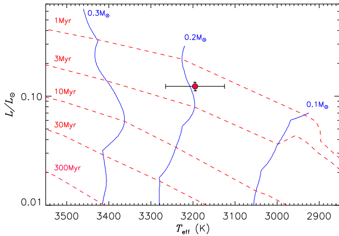
Fig. B.2. ISO-Chal 52 in the HR diagram. See Table 1 for the values of T_{\text{eff}} and L_* derived with the ROTFIT code. Isochrones and evolutionary tracks by Baraffe et al. (2015) are overplotted as dashed and solid lines; the labels represent their age and mass.
