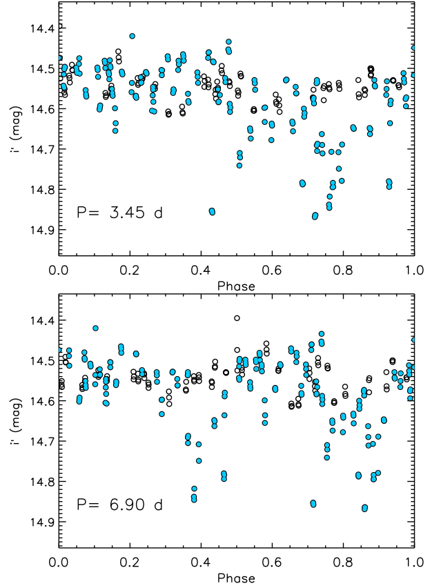
Fig. C.4. Light curve in the i' band folded in phase with the period of 3.45 days ( upper panel ) and 6.9 days ( lower panel ). Filled dots refer to the data acquired before the end of May 2019 (JD < 2458630), and open dots are related to the second part of the data (August–October 2019).
