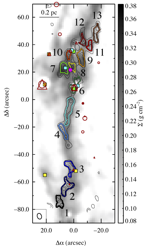
Figure 2. Highlighting the projected location of the dendrogram leaves discussed in Section 3. Each leaf is denoted with an ID number and a coloured contour. Information relating to each leaf can be found in Table 1. The background image is the mass surface density map of Kainulainen & Tan (2013) and all symbols are defined in Fig. 1.
