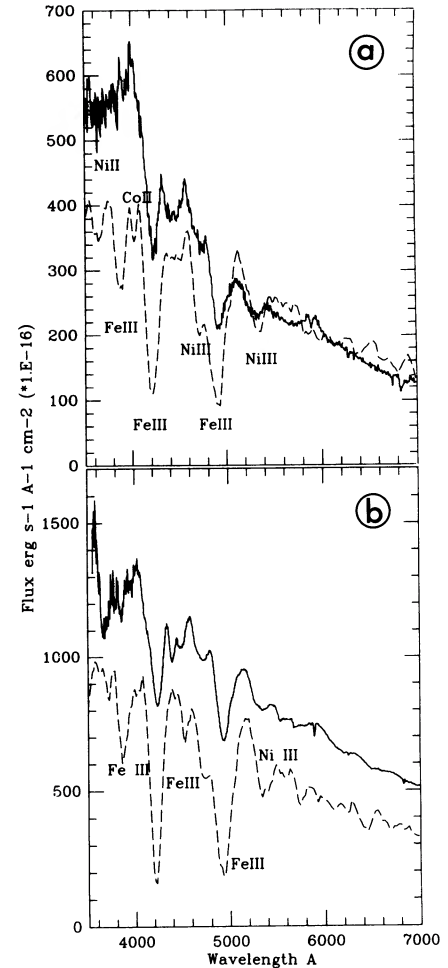
FIG. 2.—(a) Comparison of the optical spectrum of SN 1991T on April 16 with a synthetic spectrum corresponding to a mixture of Fe and Co in the proportions resulting from the decay of pure ^{56}\text{Ni} into ^{56}\text{Co} , followed by that of ^{56}\text{Co} into ^{56}\text{Fe} assuming that the explosion happened on April 10. The spectra are in the parent galaxy rest frame. The agreement in absolute flux between models and observed spectra has been imposed on the models through the assumption of the appropriate luminosity. (b) Same as 2a but for date April 20 (10 days after explosion). The observed spectrum has been shifted upward by 2 \times 10^{-14} \text{ ergs s}^{-1} \text{ cm}^{-2} \text{ \AA}^{-1} .
