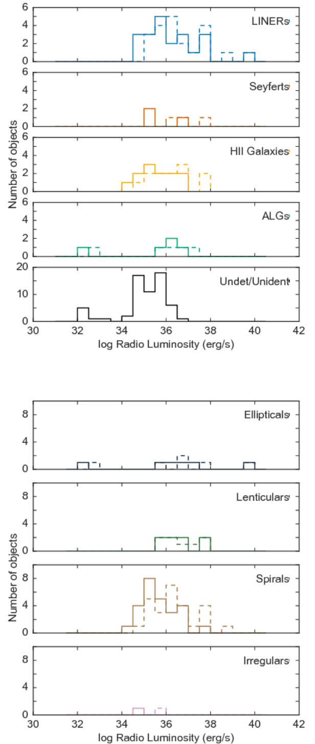
Figure 3. Histograms of the radio luminosity (erg s ^{-1} ) per optical class (upper plot) and host morphological type (lower plot). The solid-line histogram represents the radio core luminosity distribution and the dashed line corresponds to the total radio luminosity distribution. In the bottom panel of the upper plot, we also show the 3\sigma upper limit radio luminosity distribution for the undetected and unidentified sources.
