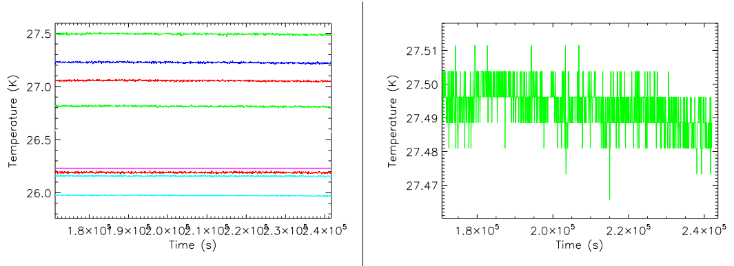
Figure 50: Behaviour of the sky load temperature during the LIS_0001 test. Left: temperature of the ECCSORB bed, right: temperature of the sky load base plate
