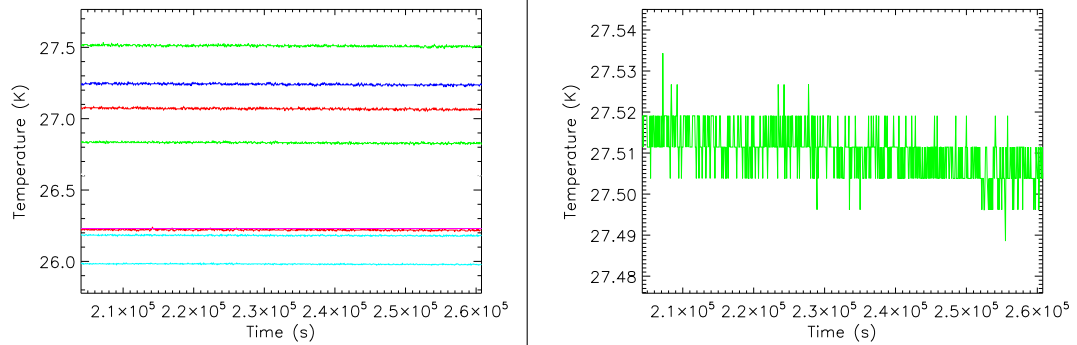
Figure 48: Behaviour of FEU temperatures during the ST1_0002 test. Left: view of all the working FPU sensors, right: detail of sensor TS2R
