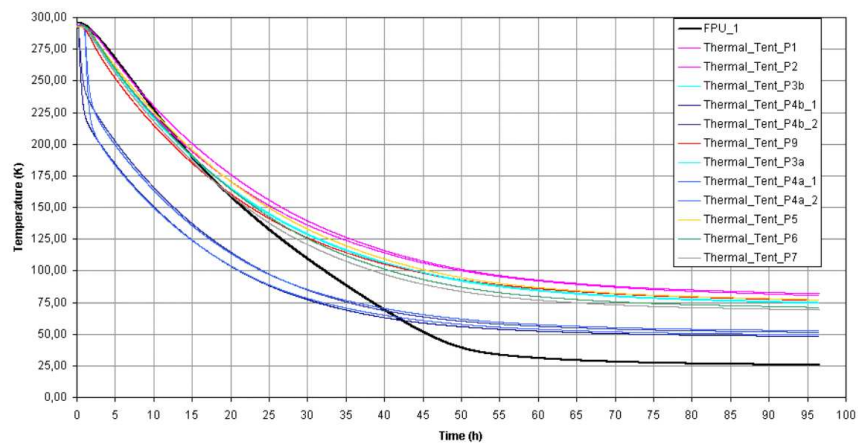
Figure 12: Measured cool-down time for the cryo-facility shroud
