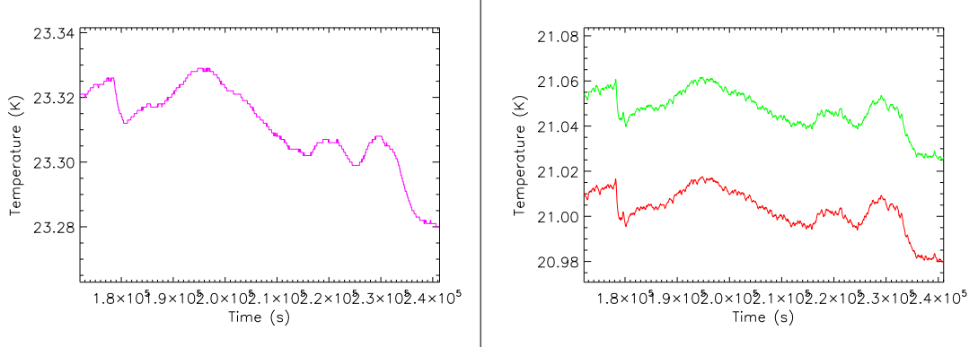
Figure 50: Behaviour of the sky load temperature during the LIS_0001 test. Left: temperature of the ECCSORB bed, right: temperature of the sky load base plate
