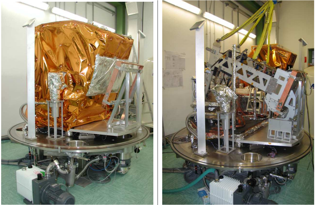
Figure 11: Left - internal view of the RAA-cryo-facility, showing the 50K internal shroud. Right - internal view of the RAA-cryo-facility when the shroud is removed and during the instrument integration.
