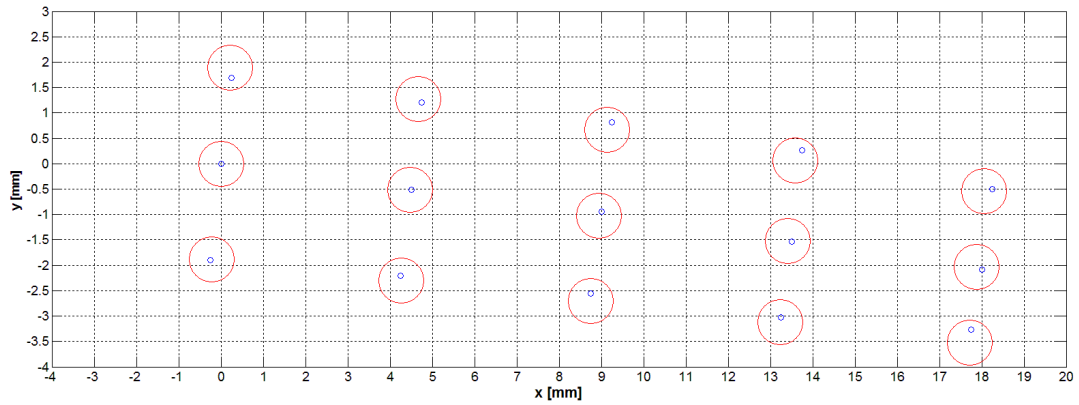
Figure 6. The red circles indicate the collimator hole projection on the tracker surface; the blue circles correspond to the hole centres reconstructed from the acquired image.
