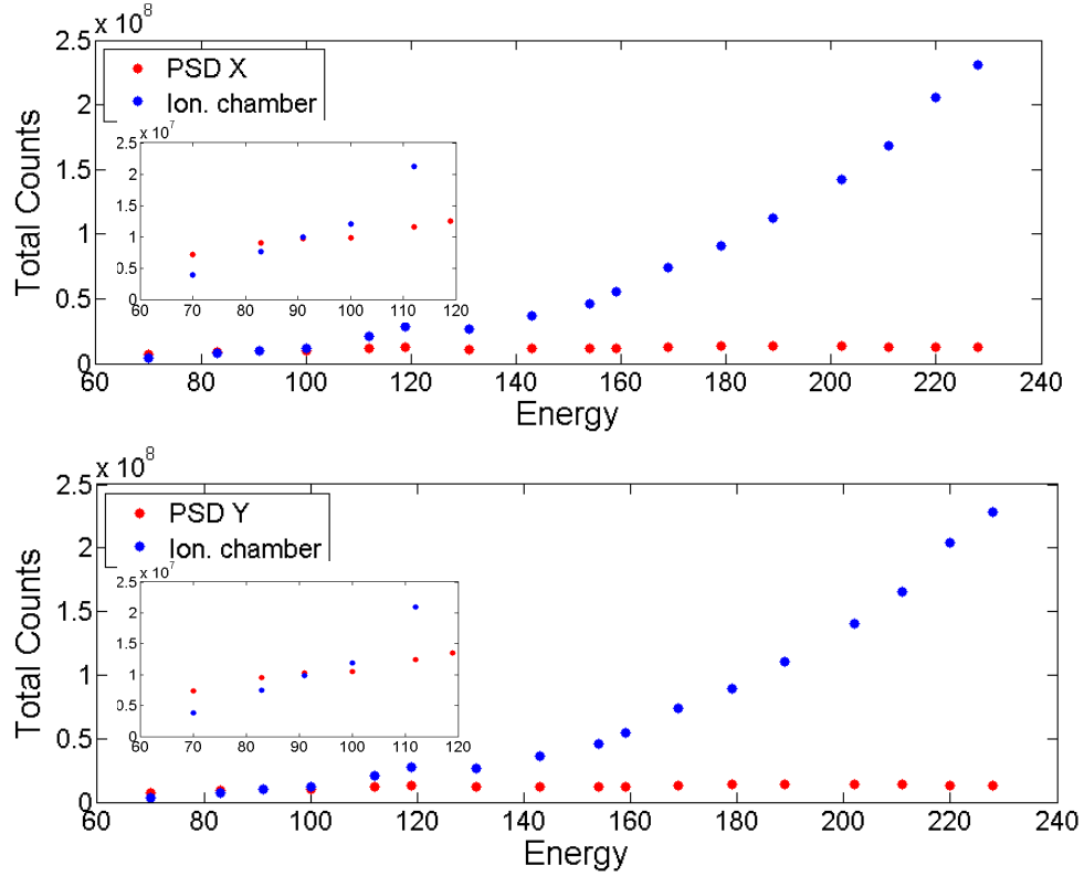
Figure 10. Red dot: fluence measured with the PSD; blue dot: fluence measured with an ionization chamber. The top panel refers to X direction and the bottom panel to Y direction.
