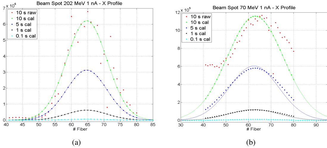
Figure 8. Examples of profiles at 202 MeV and 70 MeV before and after calibration by means of Gaussian fit of raw data.
