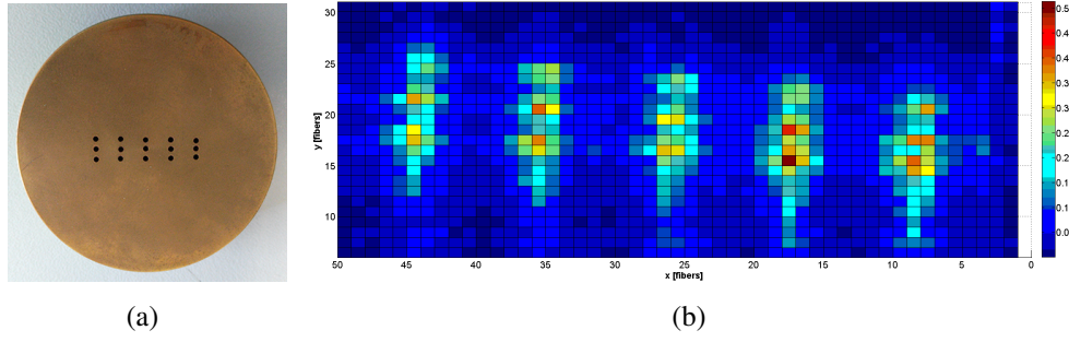
Figure 5. Image of a calibrated brass collimator with 1 mm diameter holes, whose spacing increased from 1.5 to 1.9 mm per direction.
