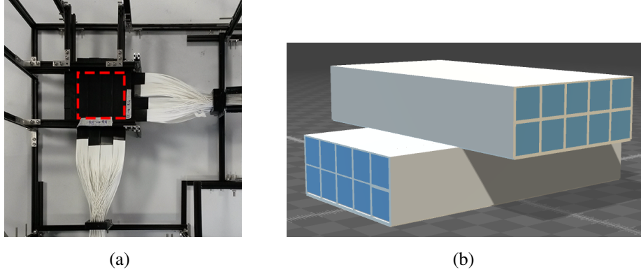
Figure 2. Front view of the QBeRT detector during the assembly phase. The dashed red box highlights the sensitive area of the detector. (b) shows a sketch of the arrangement of the four layers.
