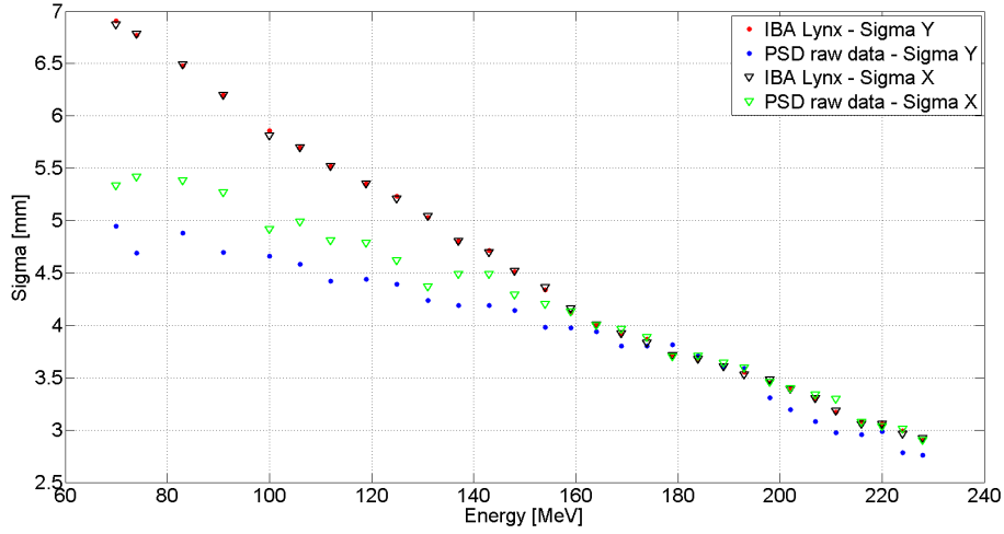
Figure 9. Comparison of measured beam spot size with the PSD and with Lynx by IBA as the sigma of the Gaussian fit of the beam profile.
