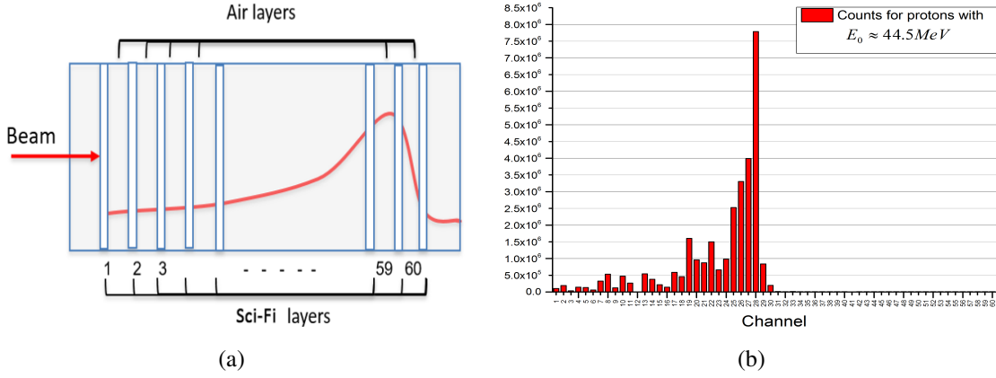
Figure 4. (a) Schematic drawing of a particle crossing the RRD. The red curve corresponds to the dose released in the detector; (b) example of signal acquired with the RRD for protons with 44.5 MeV input energy.
