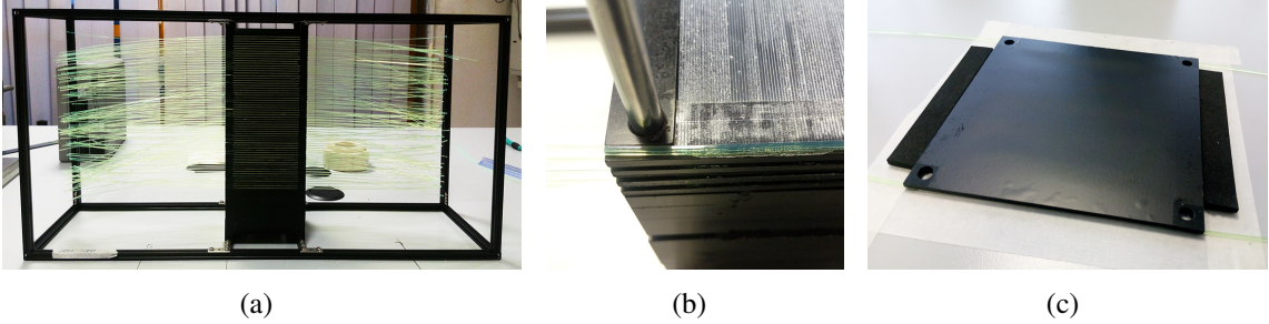
Figure 3. (a) Side view of the RRD prototype during assembly; (b), (c) different views of the RRD layers during assembly.
