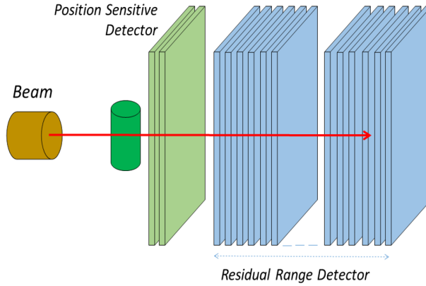
Figure 1. The layout of the QBeRT proton tracking system.
