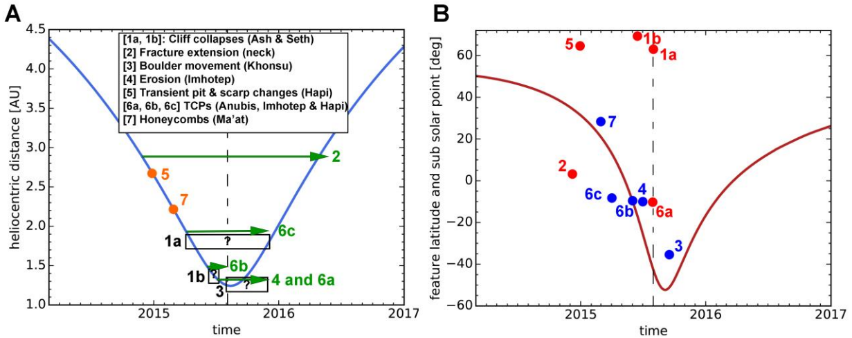
Fig. 4. Summary of event timeline versus heliocentric distance (A) and sub solar latitude [SSL] (B). The dashed line points to perihelion period. In panel A, TCPs in the legend stands for “transient circular patterns”. Orange colors represent single events of confirmed time, green arrows represent continuous activity in a given period, and black boxes represent single events where the exact time is unknown but constrained to a given period. In panel B: blue dots signify events that appear to be insolation-driven, i.e., active within \pm 20^\circ of the SSL. Red dots represent events that appear to be driven by other processes. Additional information is in table S2.
