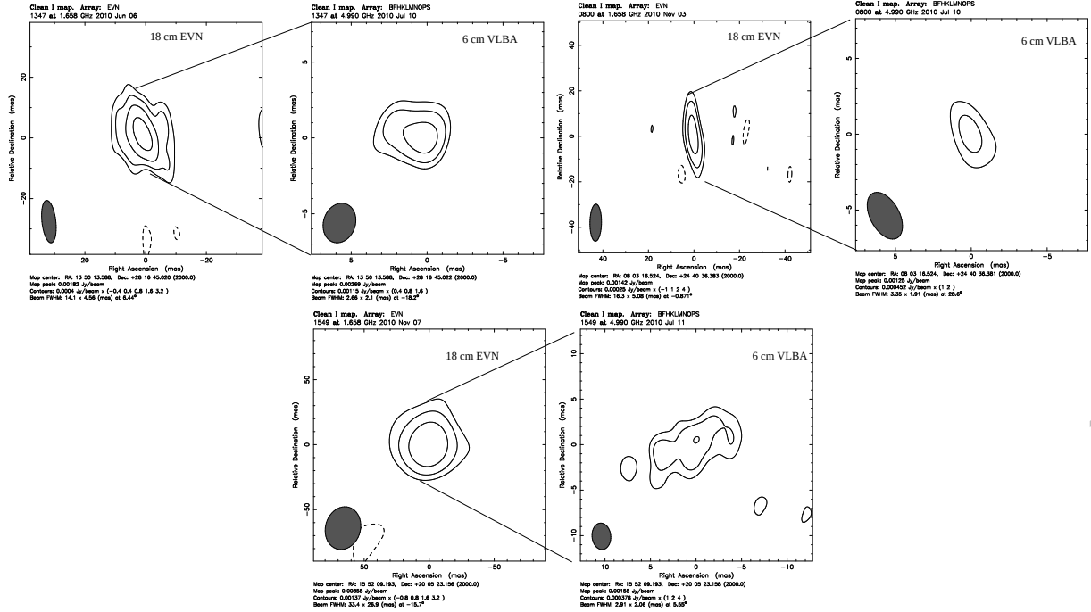
Figure 1: 18 cm EVN and 6 cm VLBA images of 3 of the faintest BCS sources recently observed.
