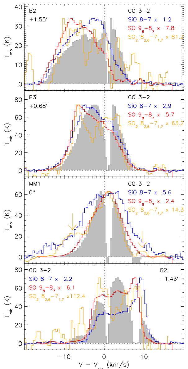
Fig. 4. Intensity profiles of SiO 8 – 7 (blue), SO 9 8 – 8 7 (red), and SO 2 8 2,6 – 7 1,7 (orange) over CO 3 – 2 (grey) at the knots (B2, B3, R2) and source (MM1) positions. The name and distance of the knots and the normalization factor to the CO 3 – 2 peak intensity are indicated in the top of the panels. The orange vertical arrows at the MM1 position indicate emission lines from complex organic molecules which are blended to the SO 2 line.
