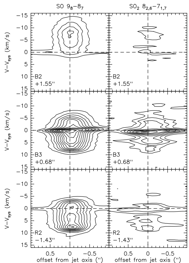
Fig. 8. From left to right: Position-velocity diagrams of SO 9_8-8_7 , and SO _2 8_{2,6}-7_{1,7} lines obtained perpendicular to the jet axis ( PA = 112^\circ ) at the position of knots B2, B3, and R2. The distance of the knots from the driving MM1 protostar is indicated. The first contour is at 5\sigma ( \sigma = 4 \text{ mJy} for SO, and 1.5 \text{ mJy} for SO _2 ) with steps of 10\sigma (SO), and 5\sigma (SO _2 ).
