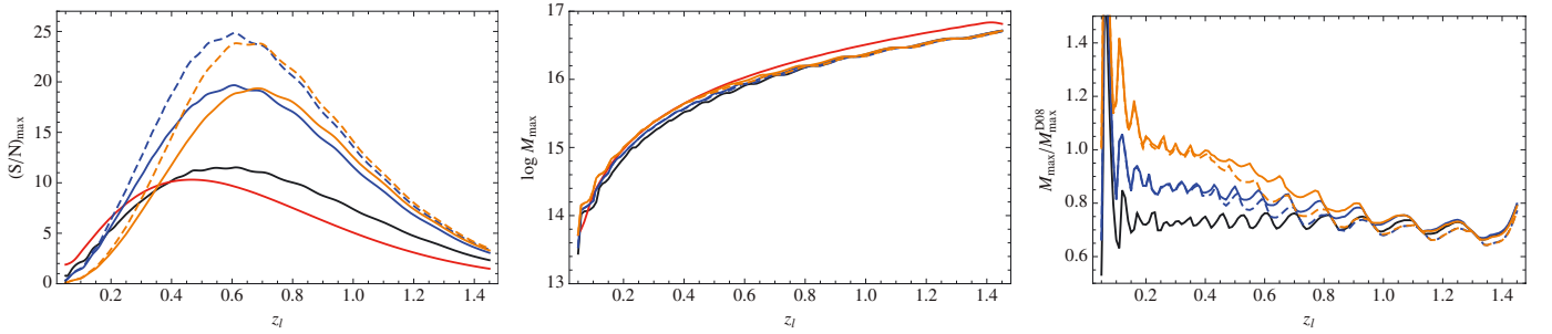
Fig. 2. Maximum S/N (left) and virial mass \log M_{\max} (centre) at which the S/N is maximised as a function of the cluster redshift. Right panel: M_{\max} normalised to the value for the D08 relation (wiggles are merely interpolation features). Black, red, blue, dashed blue, orange, and dashed orange lines refer to B01, D08, Ok10, Ok10z, Og12, and Og12z, respectively.
