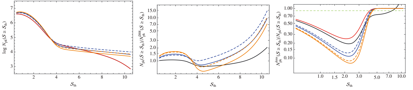
Fig. 3. Left: total number of peaks as a function of the threshold S/N S_{\text{th}} . Centre: same as before, but scaled with respect to the D08 fiducial MC relation. Right: ratio between the number of peaks due to clusters and the total one as a function of S_{\text{th}} . In each panel, black, red, blue, dashed blue, orange, and dashed orange lines refer to the B01, D08, Ok10, Ok10z, Og12, and Og12z MC relations.
