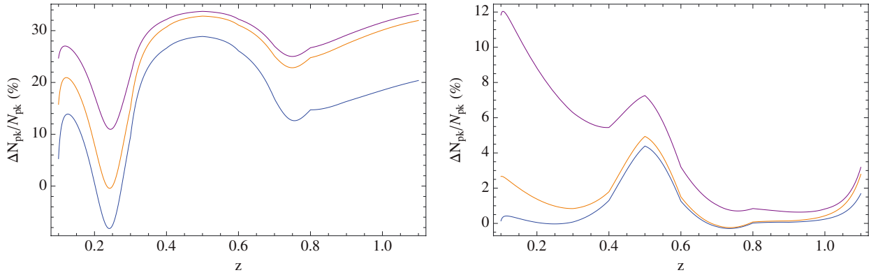
Fig. 8. Percentage deviations \Delta N_{\text{pk}}(z)/N_{\text{pk}}(z) = [\mathcal{N}_{\text{pk}}^{\text{CDM}}(z) - \mathcal{N}_{\text{pk}}^{\text{bar}}(z)]/\mathcal{N}_{\text{pk}}^{\text{CDM}}(z) of the baryons including peak number counts from the CDM-only case for the reference (blue), AGN80 (orange), and AGN85 (purple) models for peaks with S/N \geq 3 (left) or S/N \geq 5 (right).
