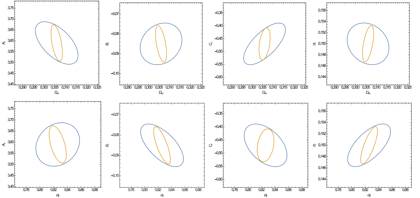
Fig. 7. Marginal error 1\sigma contours for all the combinations of MC parameters with \Omega_m (top panels) and \sigma_8 (bottom panels), for the case with (yellow curves) or without (blue curves) Planck priors.
