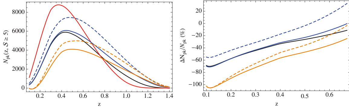
Fig. 4. Left: number of peaks with S \geq 5 in redshift bins of width \Delta z = 0.1 as a function of the bin redshift. Right: percentage deviation of the number of peaks per bin with respect to D08 (only reporting the range where N_{\text{pk}}(z, S \geq 5) for D08 is significantly non-vanishing). Black, red, blue, dashed blue, orange, and dashed orange lines refer to B01, D08, Ok10, Ok10z, Og12, and Og12z, respectively.
