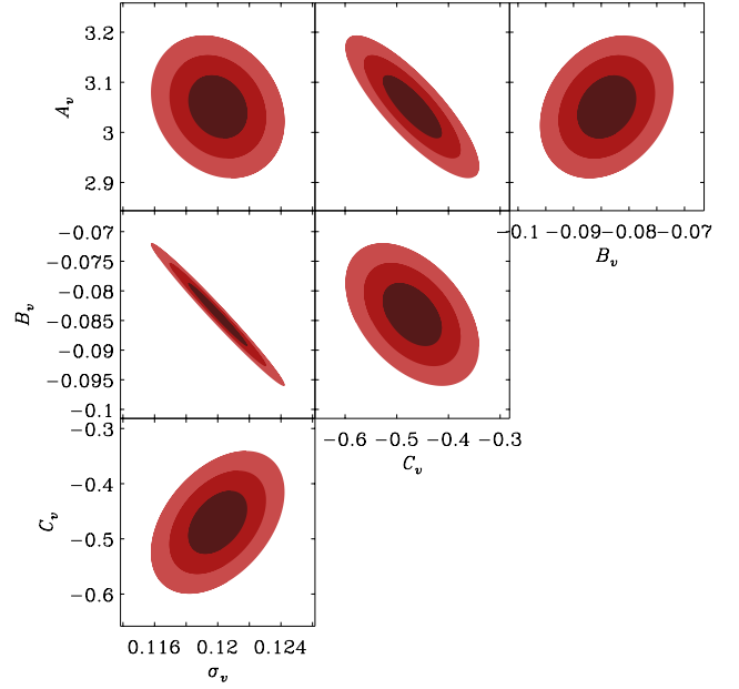
Fig. 5. Fisher matrix forecasts for the 68, 95, 99% CL assuming a fiducial D08 MC relation and a filter aperture \theta = 2 arcmin.
