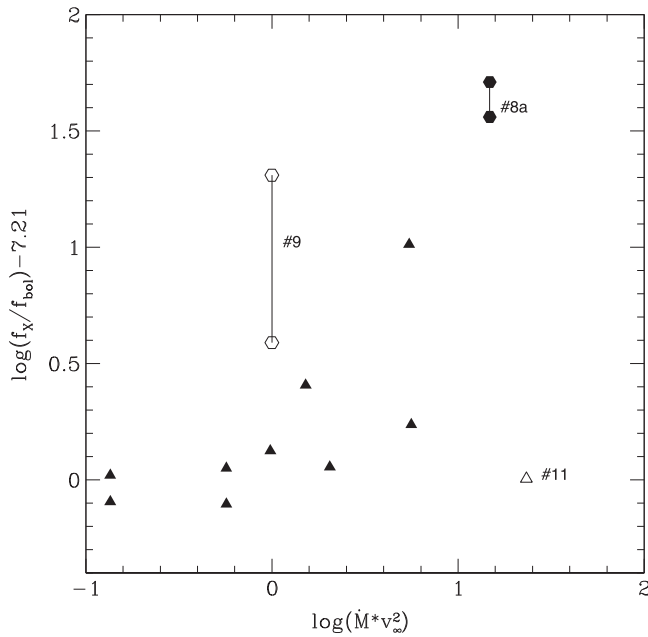
Figure 8. Overluminality in the X-ray domain versus kinetic power of the primary wind for the known binary systems in our sample. Triangles indicate Chandra ACIS-I data, while the data for Cyg OB2 #8a and 9 (hexagons) are taken from XMM-Newton observations. Filled symbols stand for systems with orbital periods of less than 30 days.
