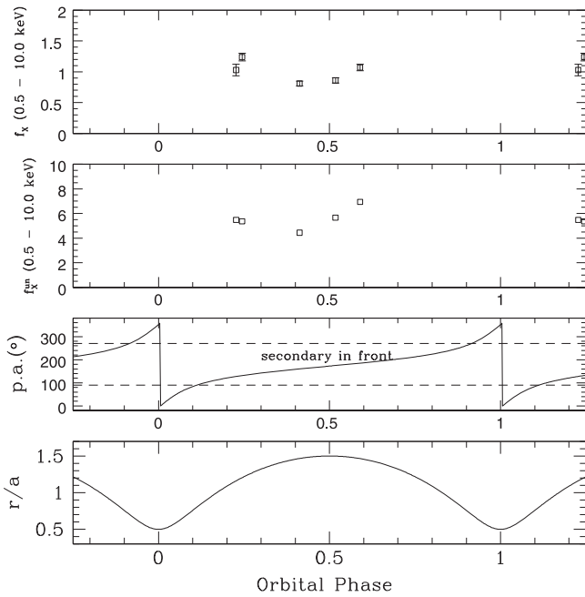
Figure 13. From top to bottom: observed and ISM-absorption corrected X-ray fluxes (in units 10^{-13} \text{ erg cm}^{-2} \text{ s}^{-1} ), position angle and relative orbital separation of Cyg OB2 #11.
