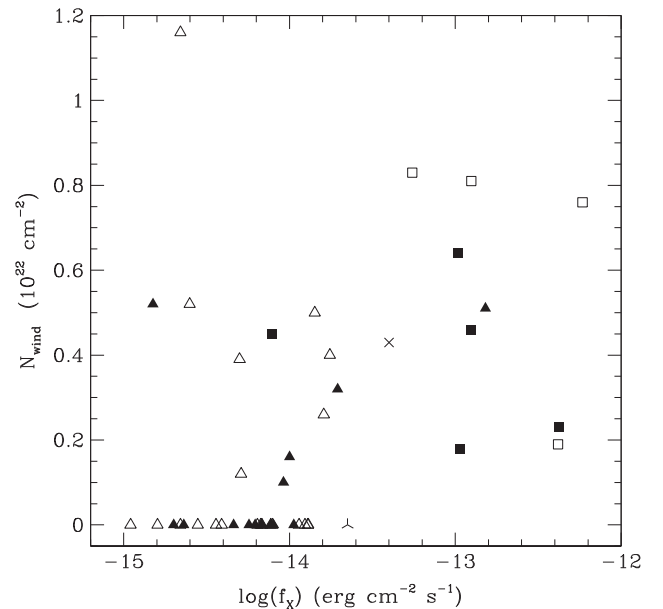
Figure 4. Left: best-fit wind column density as a function of interstellar neutral hydrogen column density. Right: best-fit wind column density as a function of observed flux in the 0.5–10 keV domain.
