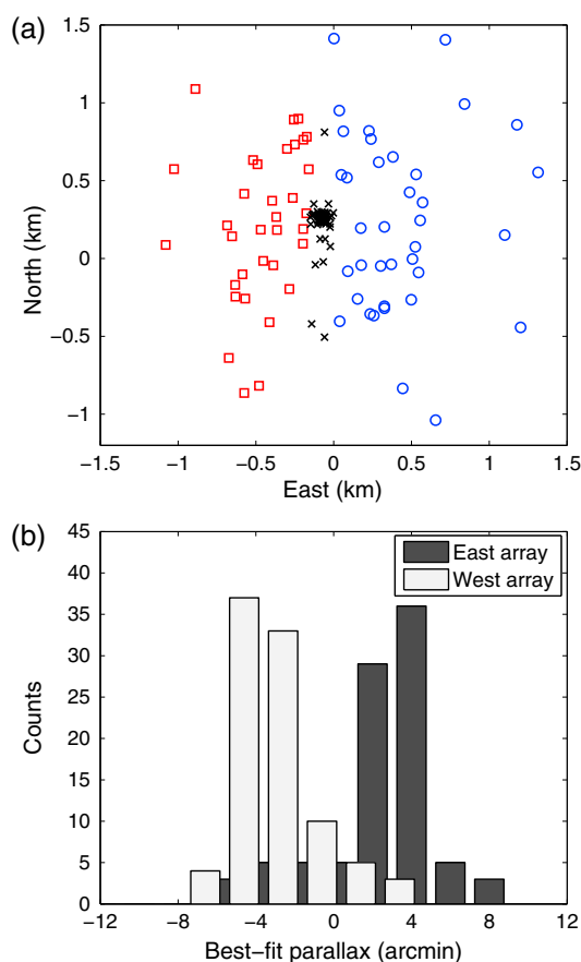
Figure 4. (a) Layout of the 128 MWA tiles, with hollow square and circle markers highlighting the two groups of tiles used for measuring the parallax shift. Central core tiles (crosses) were excluded to maximize the effective baseline ( \sim 890 m), leaving 37 tiles for the east half and 35 for the west. (b) Histograms of the parallax shifts measured for the east and west halves, each from 92 independent measurements (46 snapshots \times two instrumental polarizations). The relative displacement of the two histograms represents a parallax of 5.3 \pm 0.4 arc min.
