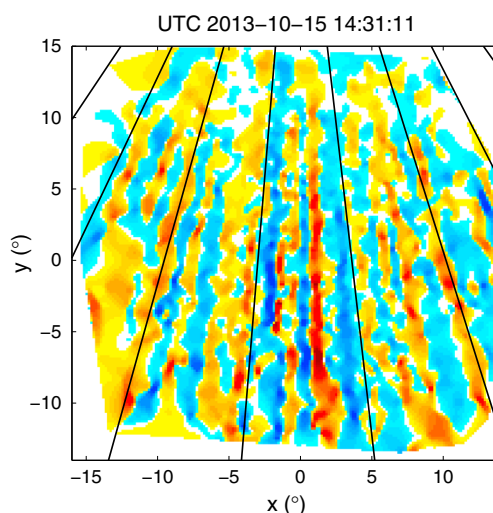
Figure 2. The vector divergence plot for the middle snapshot (i.e., the divergence of the vector field shown in Figure 1b), with the duct structure clearly visible. Positive divergence regions (relative overdensities) are represented by red-yellow hues, while negative divergence regions (relative underdensities) are represented by blue-cyan hues. White represents either values close to zero (within the FoV) or non-numeric (outside the FoV). Geomagnetic field lines have been overplotted as black solid lines, as for Figure 1.
