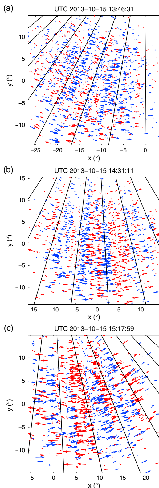
Figure 1. The vector fields of celestial source offsets for the (a) first, (b) middle, and (c) last snapshots, overplotted with the geomagnetic field lines (black solid lines) from a single L shell. Field line positions were computed based on the Australian Geomagnetic Reference Field model [Geoscience Australia, 2010] at an altitude of 600 km. Assumed to be locally straight and parallel, their apparent convergence arises from a perspective distortion due to their steep (−60°) inclination. The center of each arrow marks the time-averaged position (used as a reference point) of a celestial radio source, and the arrow represents its displacement vector. Arrow lengths have been scaled to 50 times the actual displacement distance. Blue and red denote arrows with positive and negative x components (westward and eastward), respectively. North is up and east is to the left as per the astronomical convention, and x = y = 0° marks the location of the zenith. Units along the x and y axes correspond to angular distance across the MWA FoV (1° ↔ 10 km at 600 km altitude).
