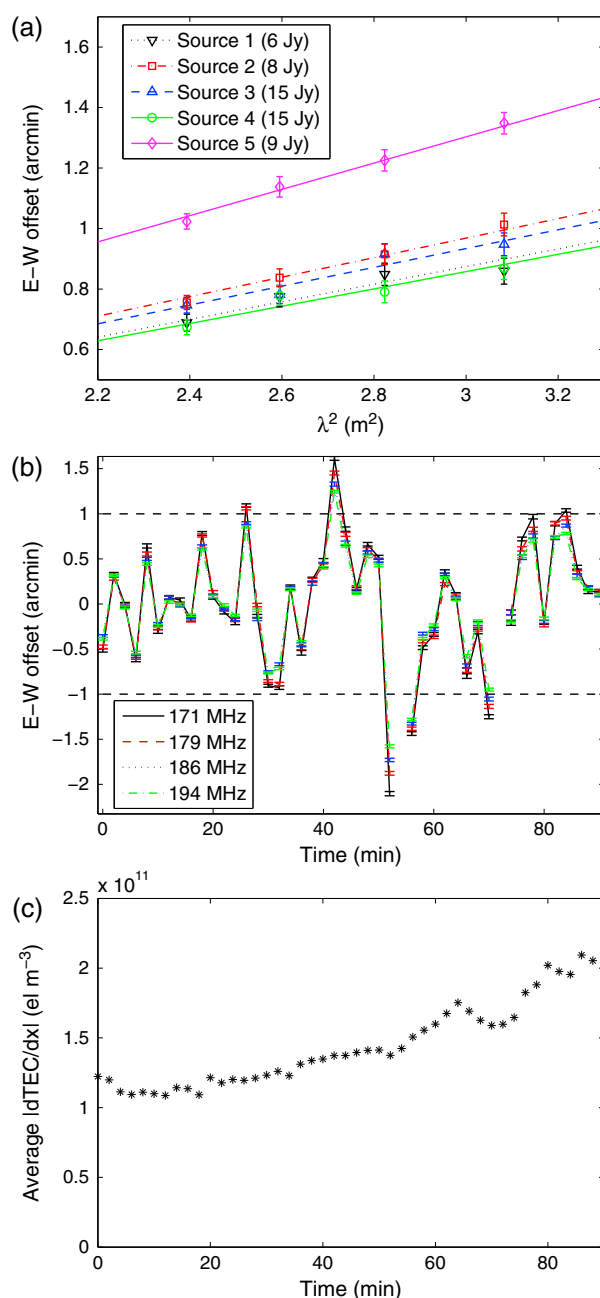
Figure 3. (a) Wavelength ( \lambda ) dependence of the size of the offset for five bright radio sources, whose flux densities are shown in the figure legend ( 1 \text{ Jy} \equiv 10^{-26} \text{ W m}^{-2} \text{ Hz}^{-1} ). Each set of points represents measurements taken in a single snapshot of time. Straight lines represent best fits to measurements at four different frequencies within the 30 MHz observing bandwidth, constrained to pass through the origin. (b) East-west component of the displacement of one of the sources in Figure 3a as a function of time. Different colors represent measurements at four independent frequencies. Dashed lines indicate the width of the telescope point spread function. Error bars in Figures 3a and 3b represent position fitting errors. (c) Time dependence of the average magnitude of the TEC gradient over all sources in a snapshot, for images formed using the full 30 MHz band.
