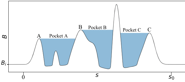
Figure 2. Situation where the magnetic field has multiple maxima along the field line. This results in multiple magnetic pockets, indicated by the shading.
