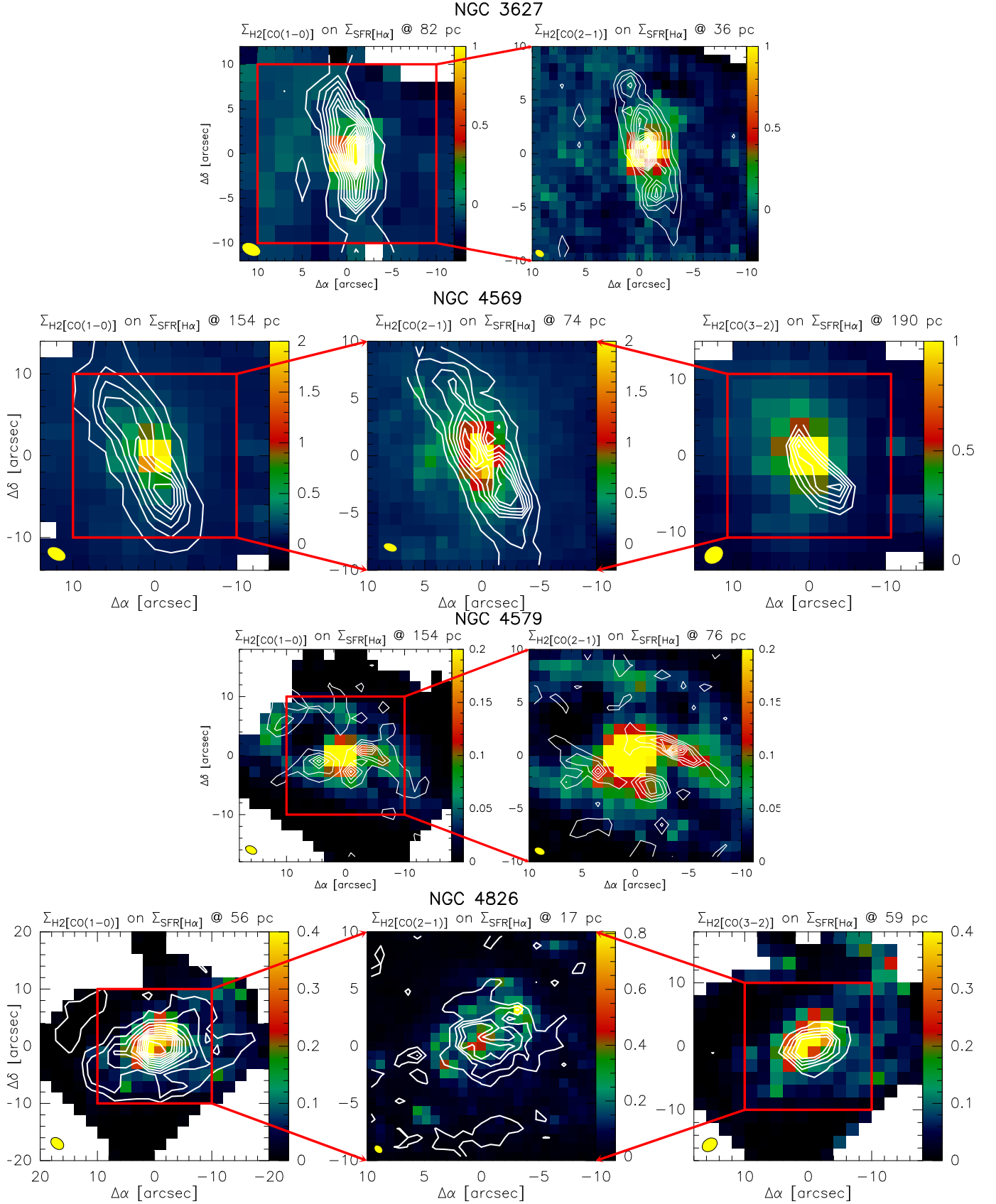
Fig. 1. \Sigma_{\text{H}_2} contours in M_{\odot} \text{ pc}^{-2} derived from ^{12}\text{CO}(1-0) , ^{12}\text{CO}(2-1) , and ^{12}\text{CO}(3-2) overlaid on \Sigma_{\text{SFR}} images in M_{\odot} \text{ yr}^{-1} \text{ kpc}^{-2} at the intrinsic spatial resolution of the ^{12}\text{CO} data and with pixel sizes equal to the ^{12}\text{CO} resolution. The beams are plotted (in yellow) in the lower left corners of maps and their values are listed in Table 2. (\Delta\alpha, \Delta\delta) -offsets are with respect to the dynamical center of each galaxy. \Sigma_{\text{H}_2} contours are drawn starting from noise levels >3\sigma with contour spacings that are whole multiples of >3\sigma .
