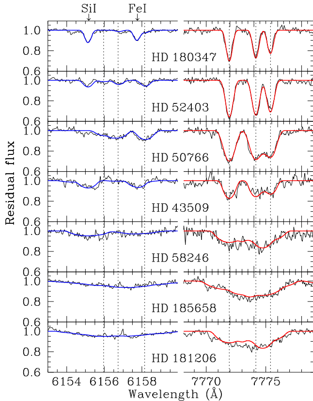
Figure 8. Left-hand side: LTE synthetic spectra computed with ATLAS9+SYNTH for O I \lambda 6155 – 8 Å triplet (blue line) overimposed with the observations (black line). Arrows on top mark the positions of two lines possibly blended with oxygen – Si I \lambda 6155.693 Å and Fe I \lambda 6157.729 Å, respectively. Right-hand side: non-LTE synthetic spectra computed with ATLAS9+SYNSPEC for the O I \lambda 7771 – 5 Å triplet (red line) overimposed with the observations (black lines). Dashed vertical lines mark the positions of triplets. Stars are ordered from top to bottom for increasing projected rotational velocities.
