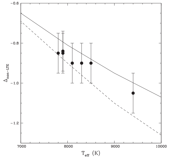
Figure 9. NLTE corrections for oxygen abundances computed for O I \lambda 7771 – 5 Å triplets. Lines represent the theoretical corrections computed by Sitnova, Mashonkina & Ryabchikova (2013) with Barklem (2007) collisional rate (solid line) and with these parameters scaled by a factor of 4 (dashed line).
