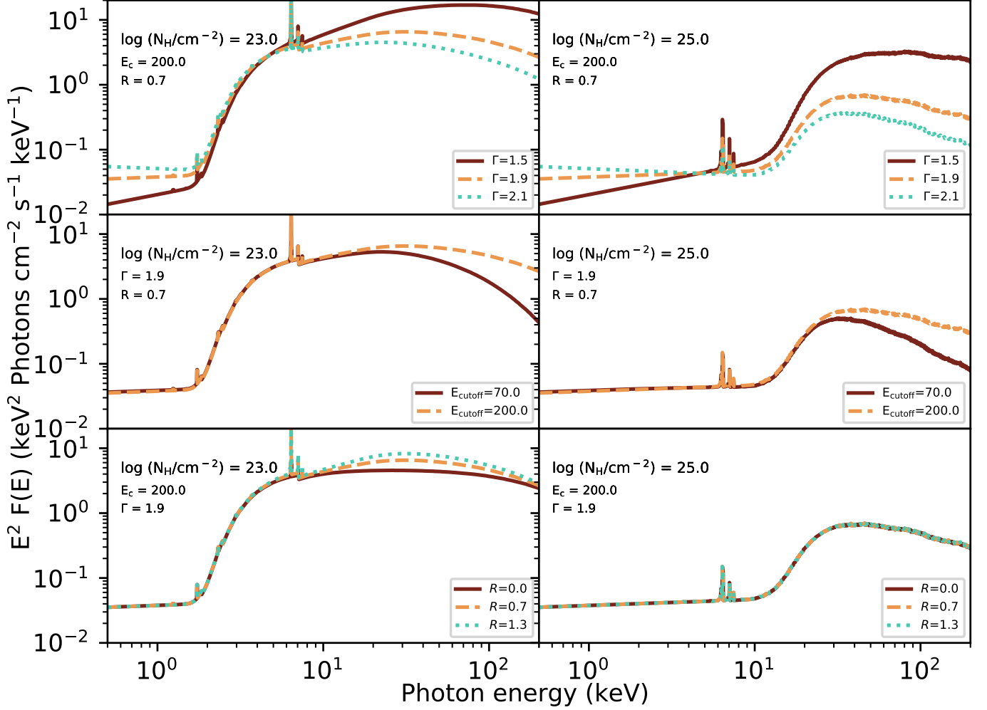
Figure 1. Dependence of X-ray spectral shape on key parameters, for two average column densities of the obscuring torus: \log(N_{\text{H}}/\text{cm}^{-2}) = 23 (left panels) and \log(N_{\text{H}}/\text{cm}^{-2}) = 25 (right panels). Top panels show three values of the power-law index, \Gamma=1.5 (solid red lines), 1.9 (dashed orange lines), and 2.1 (dotted green lines); the other spectral parameters are fixed, with scattering fraction, f_{\text{scatt}}=1\% , cutoff energy, E_{\text{cutoff}} = 200 keV, and reflection scaling factor, R = 0.7 . Middle panels show two values of the cutoff energy, E_{\text{cutoff}}=70 keV (solid red lines) and 200 keV (dashed orange lines), with f_{\text{scatt}}=1\% , \Gamma = 1.9 , and R = 0.7 . Bottom panels: three values of the reflection fraction, R=0.3 (solid red lines), 0.7 (dashed orange lines) and 1.0 (dotted green lines), with fixed f_{\text{scatt}}=1\% , \Gamma = 1.9 , and R = 0.7 . Details about the xSPEC models are given in § 3.1.
