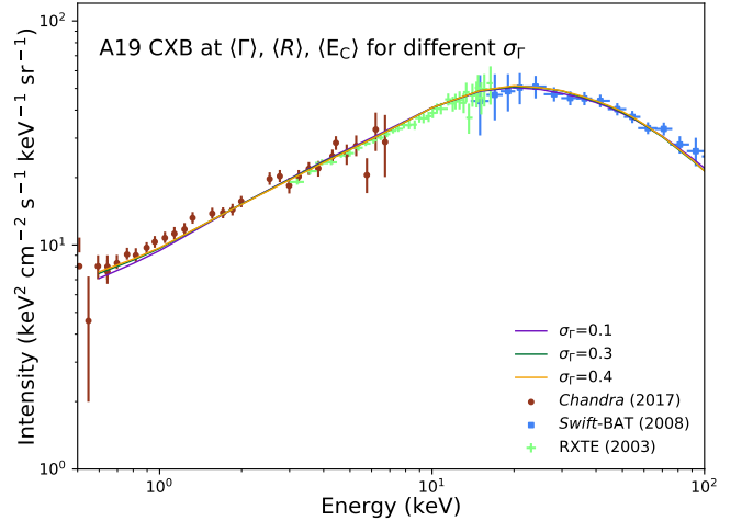
Figure 5. Fits to the CXB obtained for the XLF presented in Ananna et al. (2019) and three examples of the spectral parameters defined in Table 2 ( \sigma_\Gamma = 0.1, 0.3 and 0.4 ). The different models (solid lines) determined by the Bayesian analysis provide equally good fits, illustrating the degeneracy of the parameters. The data points are from Chandra COSMOS (Cappelluti et al. 2017; red dots), RXTE (Revnivtsev et al. 2003; bright green crosses) and Swift -BAT (Ajello et al. 2008).
