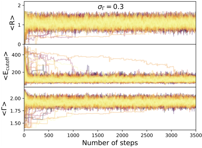
Figure 3. An example of convergence of the ensemble sampler in the Bayesian analysis part for the \sigma_\Gamma = 0.3 case. Each line represents one ‘walker’ of the ensemble sampler, which explores the parameter space to find regions that best reproduce the observed CXB.
