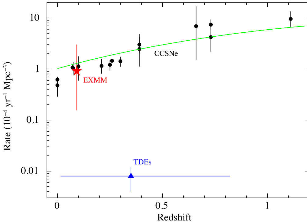
Figure 6. The core-collapse supernova data (black dots) are from Cappellaro et al. (2015, and the references therein). The green solid line shows the predicted core-collapse supernova rate from Madau & Dickinson (2014) for a Salpeter initial mass function with the lower and upper mass limits for the progenitors of 8 and 40 M_{\odot} . The blue triangle represents the rate of tidal disruption event (from van Velzen 2018).
