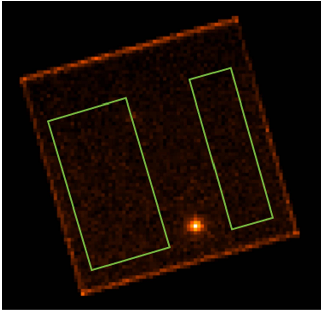
Figure 1. Small-window EPIC-pn image corresponding to the 2006 data of the double pulsar (first XMM-Newton orbit). The bright spot indicates the target, while the green rectangles show the areas selected to extract the background spectrum.
