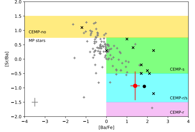
Fig. 5. [Sr/Ba] vs. [Ba/Fe] for J1907 (red filled circle), Hansen et al. (2019, black X), Hansen et al. (2018b, grey crosses), star SDSS J100714+160154 from Frebel et al. (2014, black filled circle). The areas corresponding to the CEMP classification proposed in Hansen et al. (2019) are shaded and labeled. A 0.15 dex error cross is added for reference.
