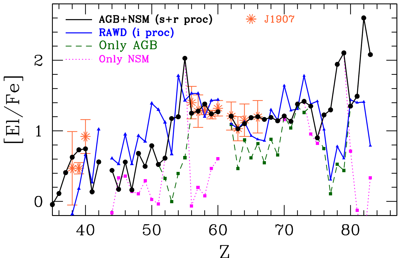
Fig. 7. The abundance pattern of J1907 compared with yields from a NSM (magenta dotted curve), an AGB star (green dashed curve), a combination of them (black solid curve) and RAWDs (blue solid curve). See text for details.
