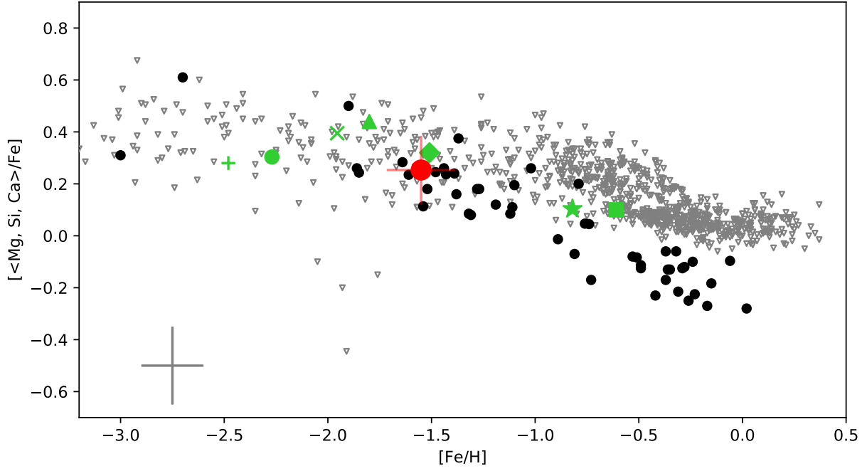
Fig. 1. [\alpha/\text{Fe}] vs. [\text{Fe}/\text{H}] for J1907 (large red circle with error bars), compared to relevant samples. Small open grey triangles, MW stars (Venn et al. 2004; Reddy et al. 2006). Black filled circles, Sgr dSph main body stars (Monaco et al. 2005; Sbordone et al. 2007; Hansen et al. 2018a, Sbordone et al., 2020 in prep.). Green large symbols, average values for globular clusters associated with Sgr dSph: square, Ter 7; star, Pal 12; diamond, NGC 6715; triangle, Arp 2; X, NGC 5634; circle, Ter 8; cross, NGC 5053 (Sbordone et al. 2005; Cohen 2004; Carretta et al. 2010; Mottini et al. 2008; Carretta et al. 2014; Sbordone et al. 2015). [\alpha/\text{Fe}] is here defined as the simple average of [\text{Mg}/\text{Fe}] , [\text{Si}/\text{Fe}] , and [\text{Ca}/\text{Fe}] , or any subsample of them available for each specific star. A reference error bar of \pm 0.15 dex on both axis is also plotted.
