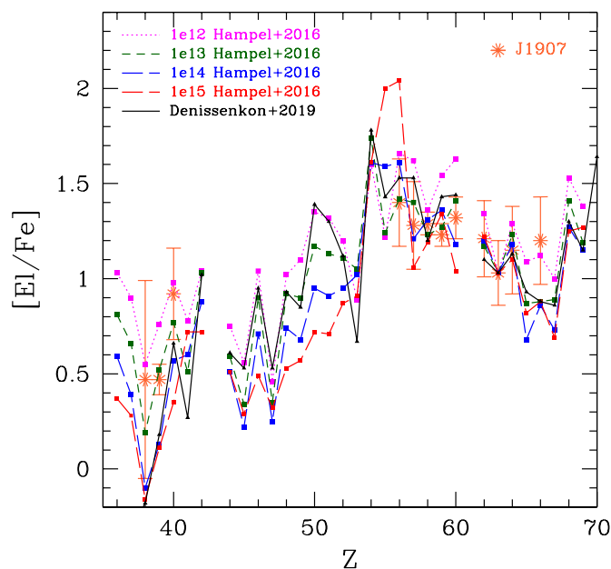
Fig. 9. i-process nucleosynthesis calculation (Hampel et al. 2016) for different neutron densities, compared to J1907. The distribution at [\text{Fe}/\text{H}]=-1.55 from Denissenkov et al. (2019) is also reported. See text for details.
