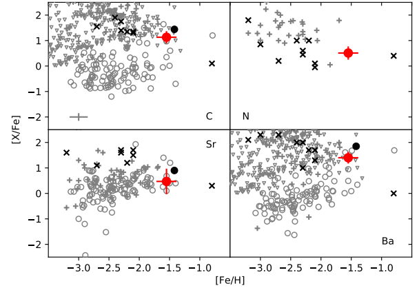
Fig. 4. [X/Fe] vs. [Fe/H] for C, N, Sr, and Ba. J1907 (red filled circle), Yoon et al. (2016, grey triangles), Hansen et al. (2019, black X), Hansen et al. (2018b, grey open circles), Allen et al. (2012, CEMP-s, -r, -s/r stars only, grey plus signs), star SDSS J100714+160154 from Frebel et al. (2014, black filled circle). A 0.15 dex error cross is added for reference. All comparison samples, except SDSS J100714+160154, belong to the MW.
