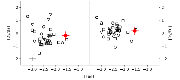
Fig. 6. [Dy/Ba] and [Dy/Eu] plotted against [Fe/H] for J1907 (red filled circle) and literature CEMP-r (triangles), CEMP-s (squares), and CEMP-rs (circles). A 0.15 dex error cross is added for reference.
