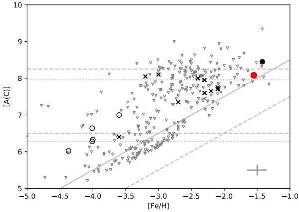
Fig. 2. A(\text{C}) vs. [\text{Fe}/\text{H}] for J1907 (red filled circle) vs. different literature samples from Yoon et al. (2016, grey triangles), Hansen et al. (2019, black X), Bonifacio et al. (2018, black open circles), star SDSS J100714+160154 from Frebel et al. (2014, black filled circle). Horizontal lines describe the high- and low-carbon band according to Spite et al. (2013, dashed), or Yoon et al. (2016, dotted). Diagonal lines are [\text{C}/\text{Fe}]=0 (dashed) and +1.0 (continuous). All comparison samples, except SDSS J100714+160154, belong to the MW.
