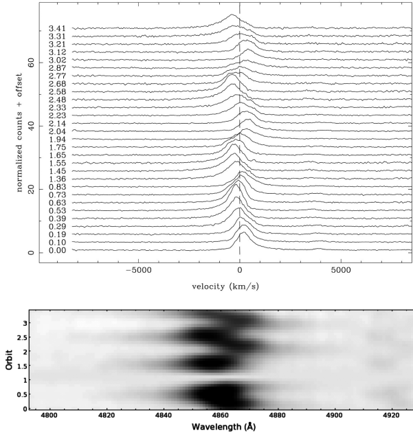
Figure 8. ESO-NTT spectra of RX J0838–2827. Top: The H_{\beta} emission line as a function of the orbital phase (computed assuming phase zero for the first NTT spectrum). Bottom: Trained spectra centred on the H_{\beta} emission line; orbital phases are relative to the 1.64-hr periodicity.
