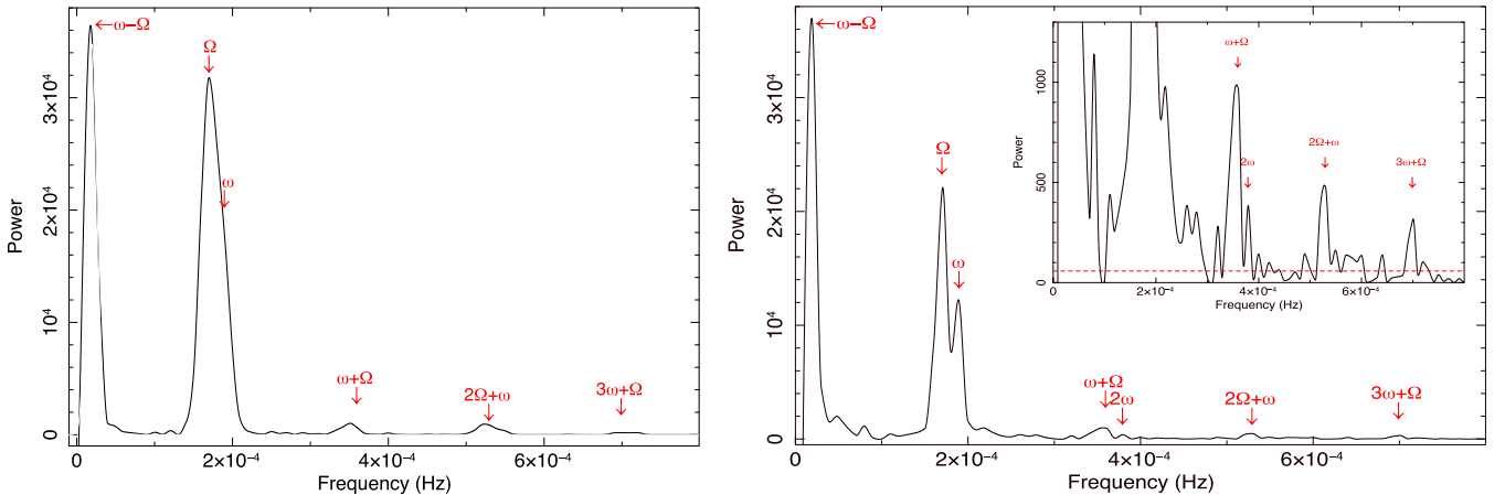
Figure 9. Power spectral distribution of RX J0838–2827 computed from the pn data of the first (left) and the second (right) XMM-Newton observations. The frequencies/peaks corresponding to the 1.64-h and 1.47-h modulations of the light-curves are identified by \Omega and \omega , respectively, and several other significant peaks can be interpreted as sidebands or higher harmonics of these frequencies (see Section 5.1). The inset is a zoom of the y-axis for purposes of clarity; the dashed line represents the 5\sigma significance threshold.
