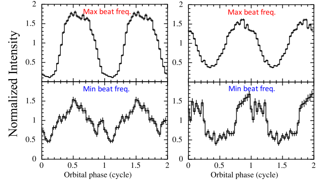
Figure 10. XMM-Newton light-curves for the first (left) and second (right) observations folded at the system orbital period. The top panels are relative to the time-span of the maximum of the beat modulation, and the bottom panels to the minimum.
