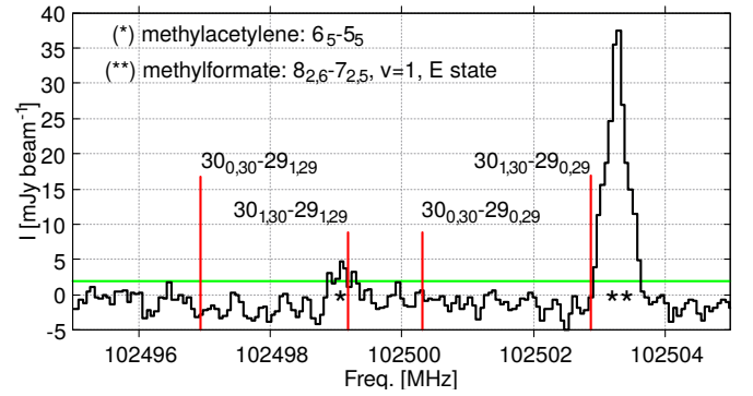
Fig. 6. Spectrum in the central beam toward the continuum peaks of IRAS 16293-2422 B. Predicted 30_{x,30} - 29_{x,29} transition lines of aG'Ag-12BD are overlaid as red sticks. The X-axis represents the frequencies in the rest frame of the system (i.e., corrected for the system V_{\text{LSR}} of 2.7 \text{ km s}^{-1} ; Jørgensen et al. 2011). The green line is an indication of the rms level ( 1.89 \text{ mJy beam}^{-1} ) represented by a spectrum extracted from an off source position.
