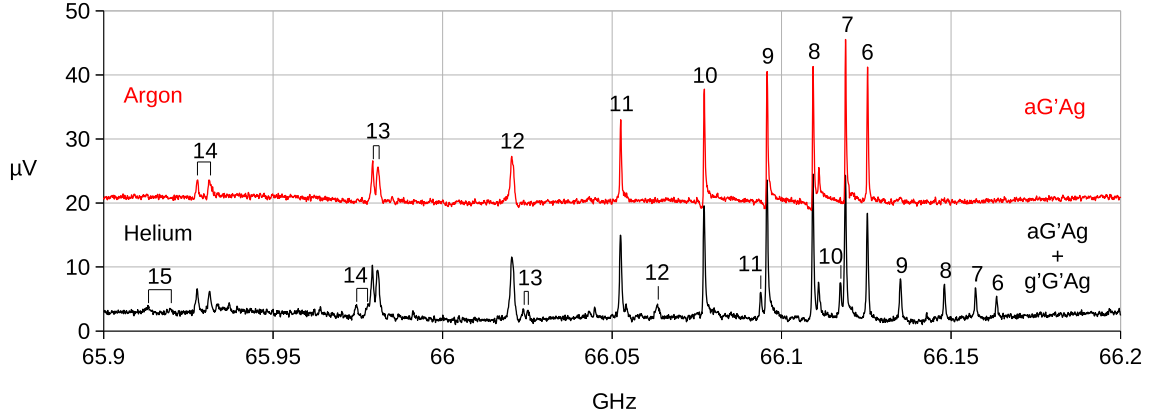
Fig. 4. Comparison between the 65.9–66.2 GHz spectra recorded using Ar (upper black red) and He (lower black trace) as carrier gas. In both spectra the aG'Ag-12BD K_a = 6 \leftarrow 5 Q -branch transitions can be recognized, whereas the same transitions of less stable g'G'Ag-12BD are completely depleted in the Ar spectrum. Numbers above the peaks indicate the assigned J quantum numbers.
