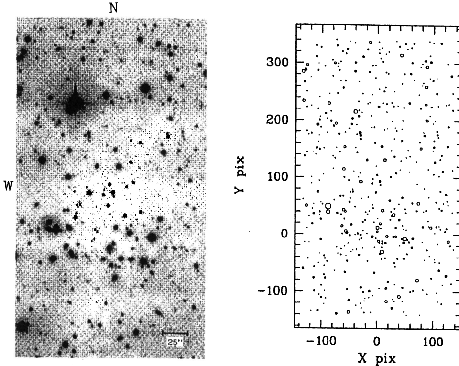
Fig. 1. g) Composite g, r, i image of S0781B and X, Y plot of the photometric catalog
