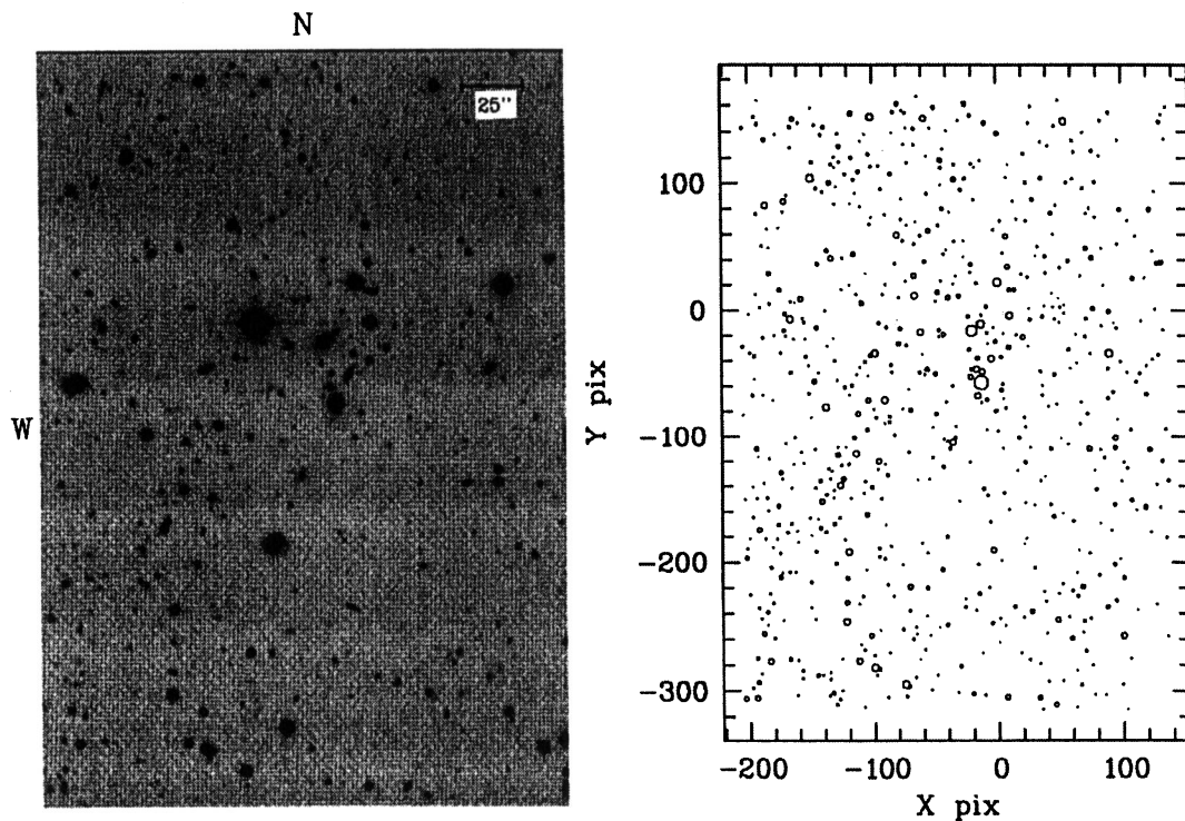
Fig. 1. a) Composite g, r, i image of MRC0254-274 and X, Y plot of the photometric catalog
