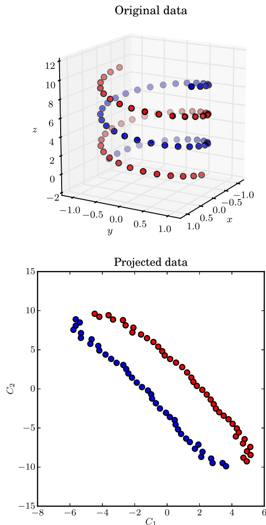
Figure A1. t-SNE projection of a double helix into two dimensions. All information about the shape of the structure is lost, but two strands become separated. Colours are used for the illustration purposes only and are not part of the data set, meaning that t-SNE only knows the coordinates of the points, regardless the colour.
