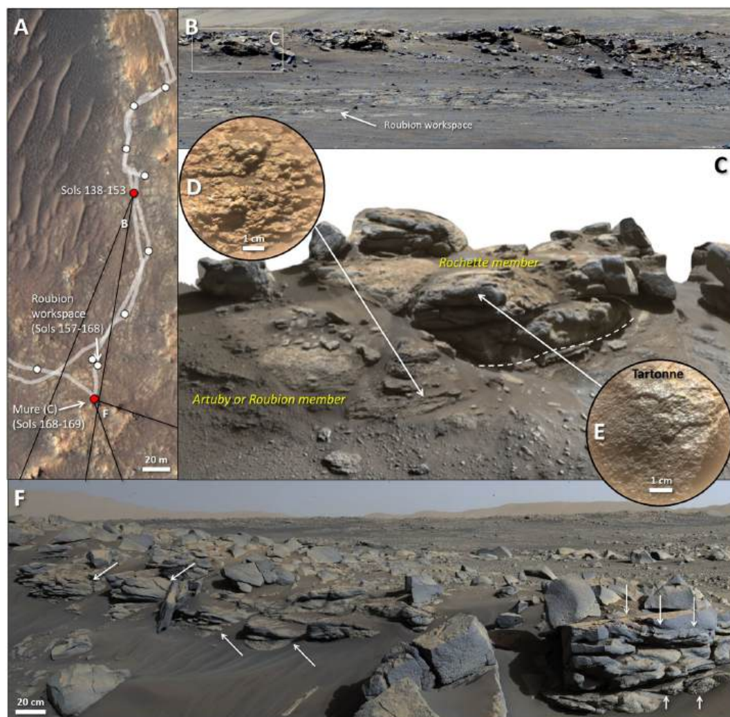
Figure 9. Observations of Mure and adjacent outcrops extending from Artuby ridge. (a) Orbital context showing the context and extent of imaging shown in (b–f). (b) Mastcam-Z enhanced color view of the Artuby ridge, specifically the Mure outcrop (c), and the context for the future Roubion sampling location (sol 143, zcam08151; NASA/JPL-Caltech/ASU/MSSS/C. Rojas). (c) 3D model of the Mure outcrop using Mastcam-Z data (sol 168, NASA/JPL/MSSS/ASU/Cornell/C. Tate), with a white dashed line delineating the Rochette member on top of the Artuby or Roubion member. (d) Supercam RMI of the Baume target, representative of the Artuby member (sol 169, scam04169). (e) Supercam RMI of the Tartonne target, representative of the Rochette member (sol 169, scam05169). (f) Mastcam-Z enhanced color view of the outcrops to the east of Mure (a), with arrows indicating examples of layering and vesicular textures (sols 168–169, zcam08180 and zcam 08181; NASA/JPL-Caltech/ASU/MSSS/K. Powell).
