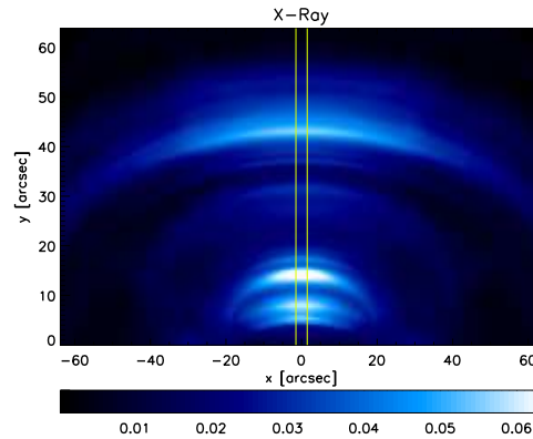
Figure 2. Upper hemisphere of an X-ray intensity map (1 keV) at t = 950 yr. Color scale is linear and in units of \text{mJy/arcsec}^2 . Vertical lines near the polar axis define the slice used in the analysis of wisp profiles.
