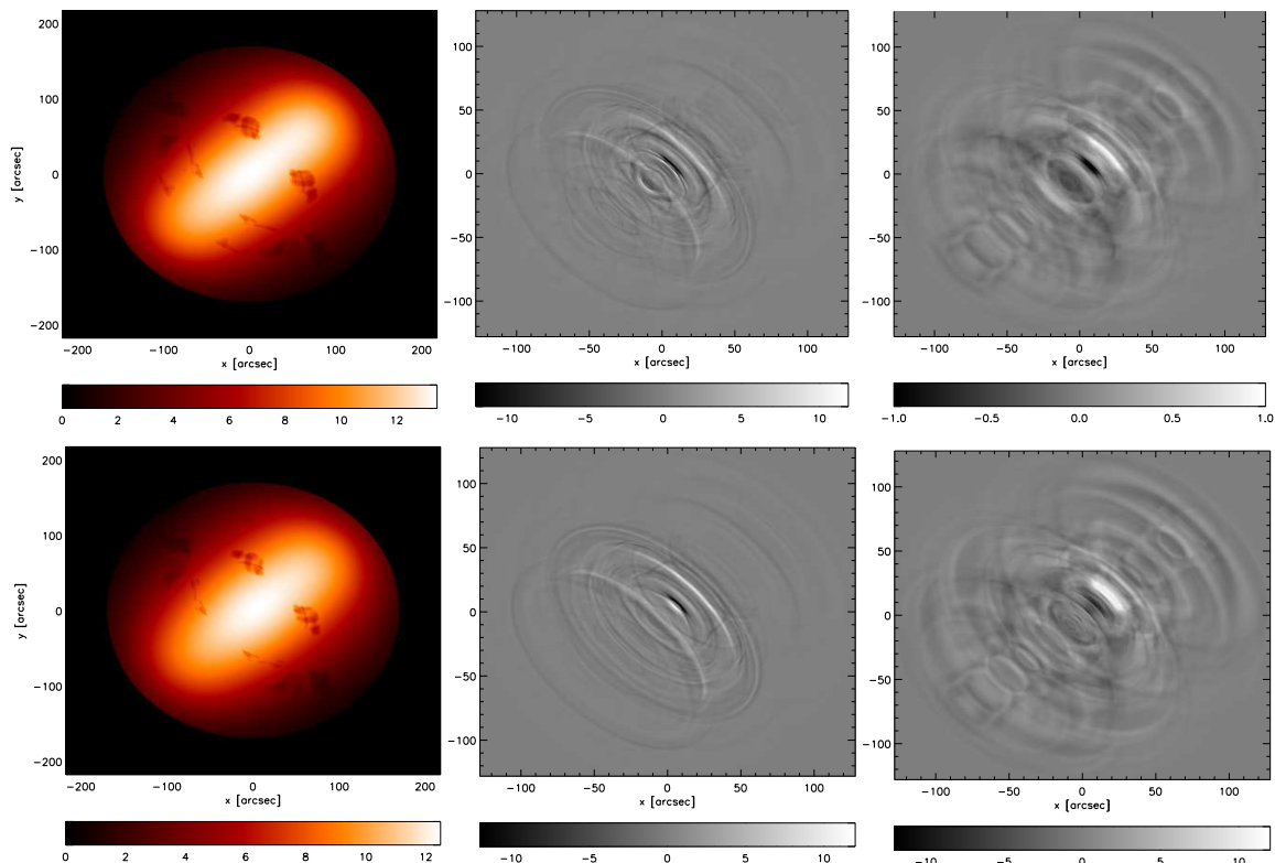
Figure 1. Radio surface brightness maps at 1.4 GHz, in units of \text{mJy/arcsec}^2 . In the upper row maps for case (A) are shown, while case (B) is in the bottom. In the left panel, emission maps with the small scales subtracted are shown for both cases. In the central and rightmost panels maps of short and long time scales wisp variability are presented.
