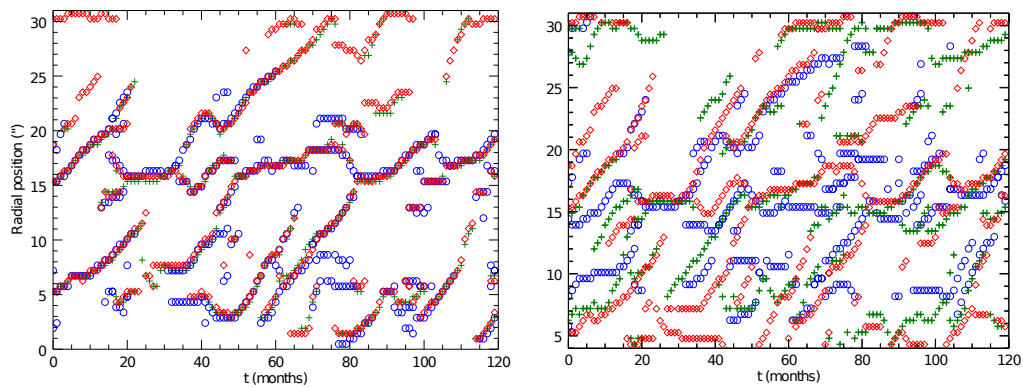
Figure 3. Radial positions of the local intensity maxima (in arcseconds) as a function of time (in months) with red diamonds identifying radio wisps ( \nu_r = 5 GHz), green crosses optical ones ( \nu_o = 3.75 \times 10^{14} Hz) and blue circles for X-rays (1 keV). On the left case (1) is shown. On the right case (3) is shown, with X-ray particles injected in the equatorial zone and radio ones injected in the complementary sector.
