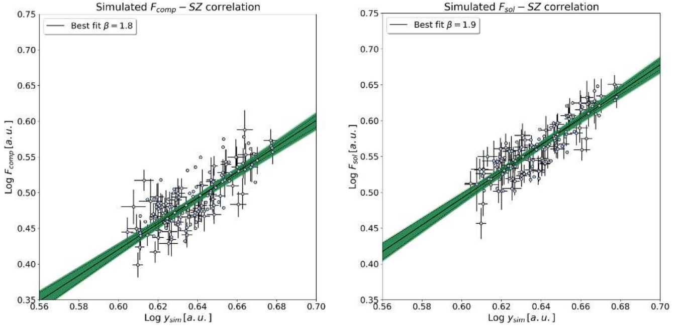
Figure 19. Left panel: F_{\text{Comp}} -SZ correlation from simulated data. Right panel: F_{\text{Sol}} - SZ correlation from simulated data.
