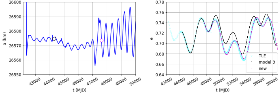
Figure 6: On the left, a close-up view of the semi-major axis evolution given by TLE for Molniya 2-10 (orbit #2). In black, the initial condition in semi-major axis used for the propagation shown in Fig. 3; in magenta the new initial condition whose propagation matches the behavior given by the TLE. On the right, the eccentricity evolution for the two propagations and the one given by TLE.
