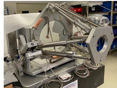
Hexapode for moving the Detector Assembly (made for Leonardo by SYMETRIE in France)
