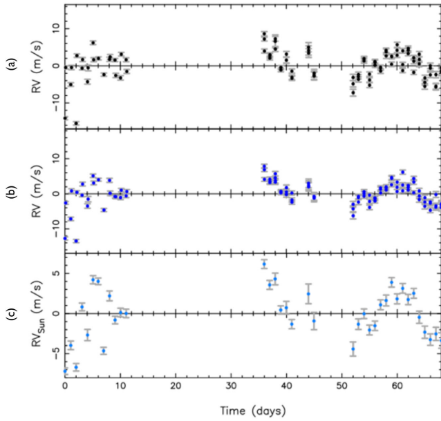
Figure 2. (a) HARPS RV variations in the solar rest frame, corrected for relativistic Doppler effects (but not yet corrected for Vesta’s axial rotation). (b) HARPS RV variations of the Sun as a star (after removing the RV contribution of Vesta’s axial rotation). (c) Nightly binned HARPS RV variations of the Sun as a star – note the change in scale on the y-axis. The values for each time series are provided in the Supplementary Files that are available online.
