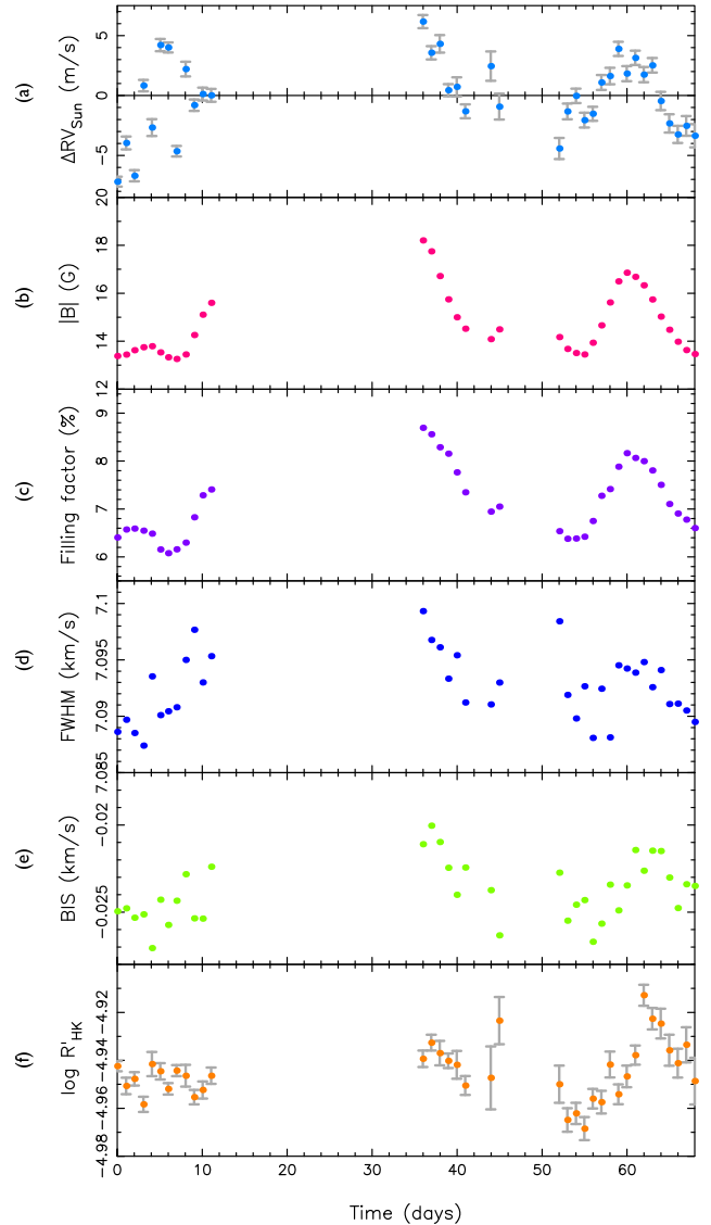
Figure 11. (a) HARPS RV variations of the Sun as a star. (b and c) Time series of the disc-averaged line-of-sight magnetic flux |\hat{B}_{\text{obs}}| and filling factor f , respectively, determined from the SDO/HMI magnetograms. (d–f) Time series of the FWHM, BIS and \log(R'_{HK}) , respectively, determined from the HARPS DRS reduction pipeline. The values of these nightly binned time series are provided in the Supplementary Files available online.
