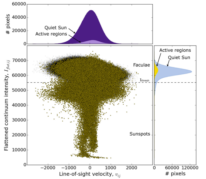
Figure 5. Pixel line-of-sight velocity, v_{ij} (in \text{m s}^{-1} ), as a function of flattened intensity I_{\text{flat},ij} , for the Sun on 2011 November 10 at 00:01:30 UTC. The top and right histograms show the distributions of v_{ij} and I_{\text{flat},ij} , respectively, in bins of 1000. In the case of active pixels (yellow dots), the line-of-sight velocity is invariant with pixel brightness. For quiet-Sun pixels (black dots), however, brighter pixels are blueshifted while fainter pixels are redshifted: this effect arises from granular motions.
