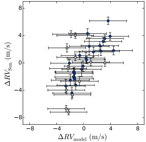
Figure 9. HARPS RV variations of the Sun as a star versus our model derived from SDO/HMI images. Observations from the first part of the run are highlighted in a lighter shade.
