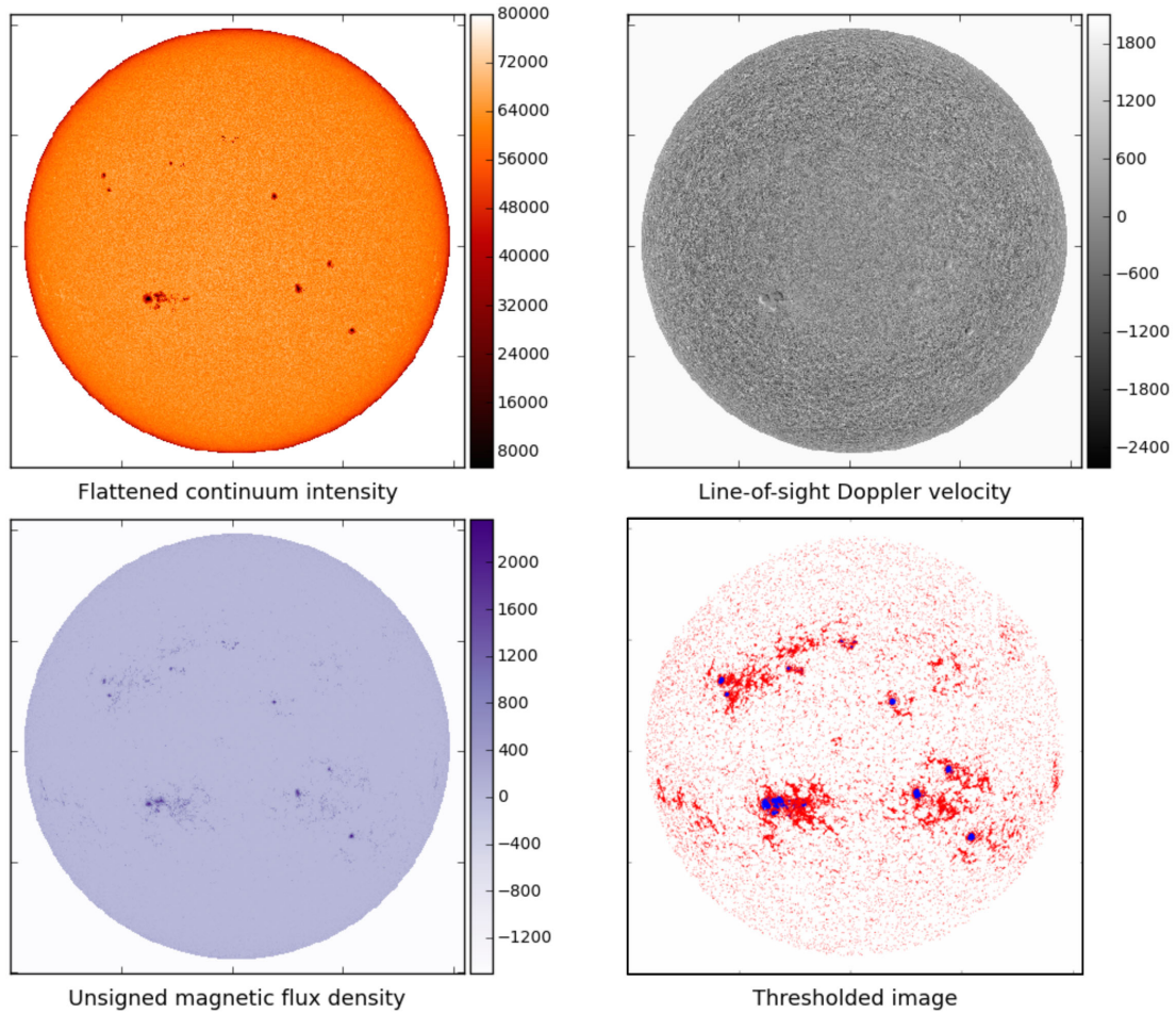
Figure 3. First three panels: SDO/HMI flattened intensity I_{\text{flat}} , line-of sight velocity v ( \text{km s}^{-1} ) for the non-rotating Sun and unsigned radial magnetic flux |B_r| (G) of the Sun, observed on 2011 November 10 at 00:01:30 UTC. Last panel: our thresholded image, highlighting faculae (red/lighter shade pixels) and sunspots (blue/darker shade pixels). For this set of observations (representative of the whole run), faculae account for 9 per cent of the total pixel count, while sunspots account for less than 0.4 per cent. The remaining \sim 90 per cent of the pixels on the solar disc are magnetically quiet.
