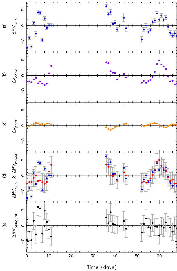
Figure 8. (a) HARPS RV variations of the Sun as a star, \Delta RV_{\text{Sun}} . (b) Scaled basis function for the suppression of convective blueshift, \Delta \hat{v}_{\text{conv}} , derived from SDO/HMI images. (c) Scaled basis function for the rotational Doppler imbalance due to spots and faculae, \Delta \hat{v}_{\text{phot}} . (d) Total RV model, \Delta RV_{\text{model}} (red/lighter shade, with errors including additional variance s ), overlaid on top of the HARPS RV variations (blue/darker shade points). (e) Residuals obtained after subtracting the model from the observations. All RVs are in \text{m s}^{-1} . Note that the scale of the y-axis is different from that used in Fig. 2. The values of these nightly binned time series are provided in the Supplementary Files available online.
