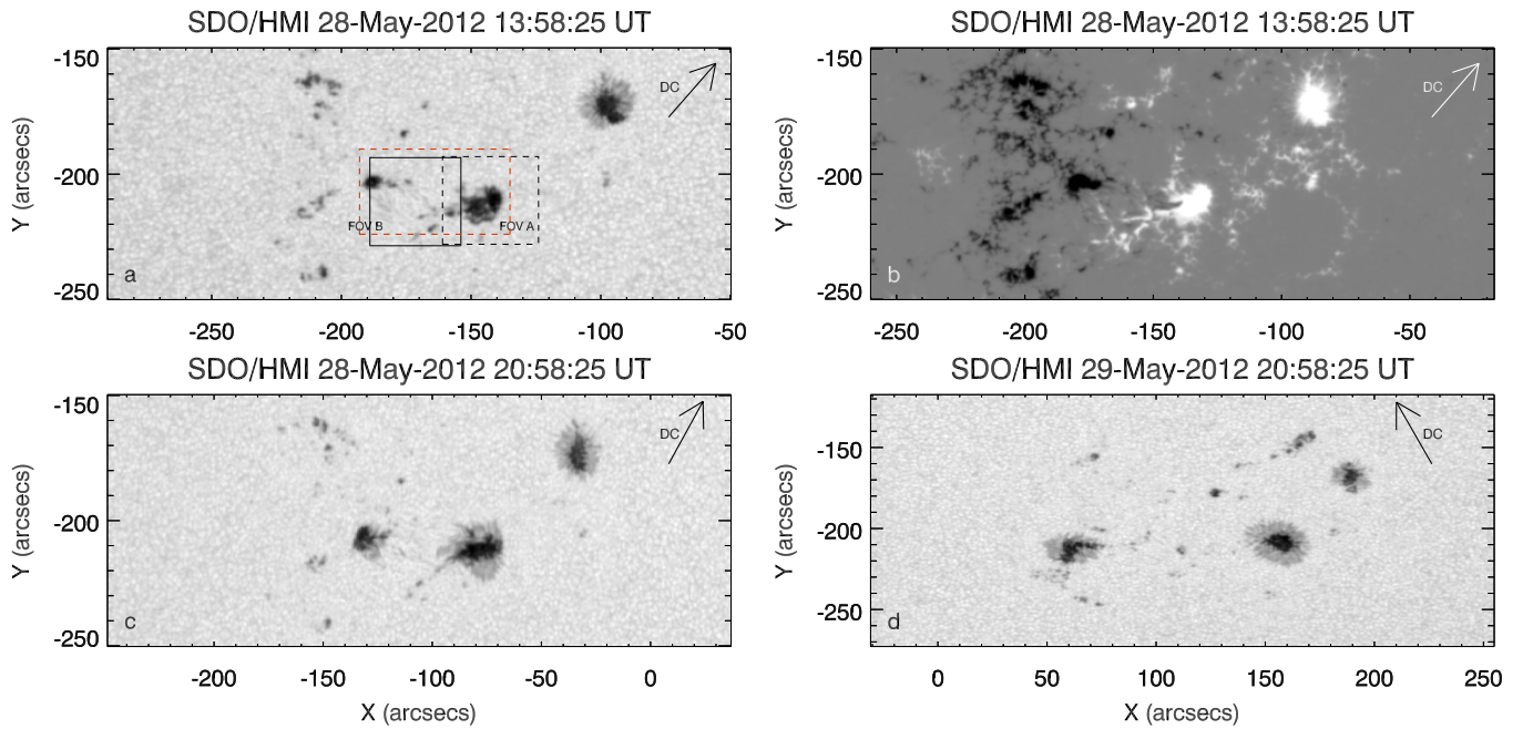
Figure 1. (a, c, d) Continuum filtergrams and (b) LOS magnetogram taken by SDO/HMI showing maps of NOAA AR 11490 at different times. The black dashed and continuum boxes in panel (a) indicate the IBIS FOVs containing the leading and the following spots, respectively, while the red box indicates the FOV shown in Figure 2. Here and in the following figures, north is at the top, and west is to the right. The axes give the distance from solar disk center. The arrow points to the disk center.
