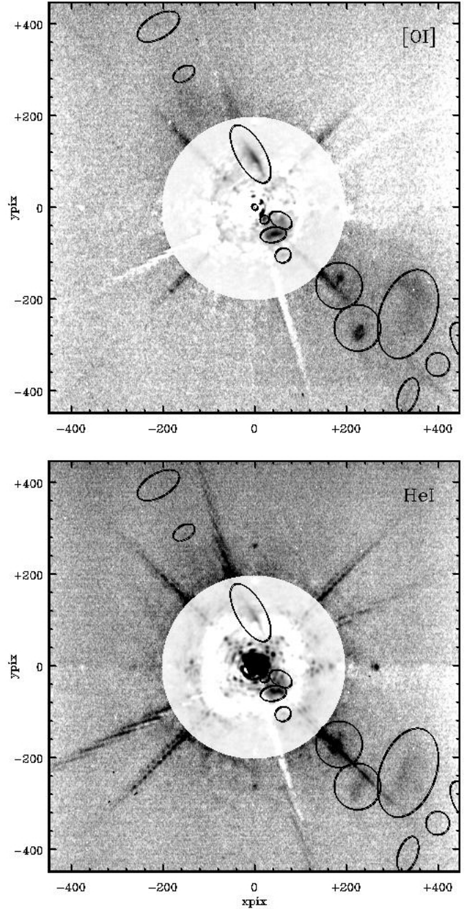
Fig. 11. SPHERE/ZIMPOL OI_630- and HeI-filter observations of the R Aqr jet. The emission of the red giant is strongly reduced by subtracting a scaled CntHa filter image. The gray scale tables are multiplied by a factor of ten for the inner r_{\text{RG}} < 0.72'' region.
